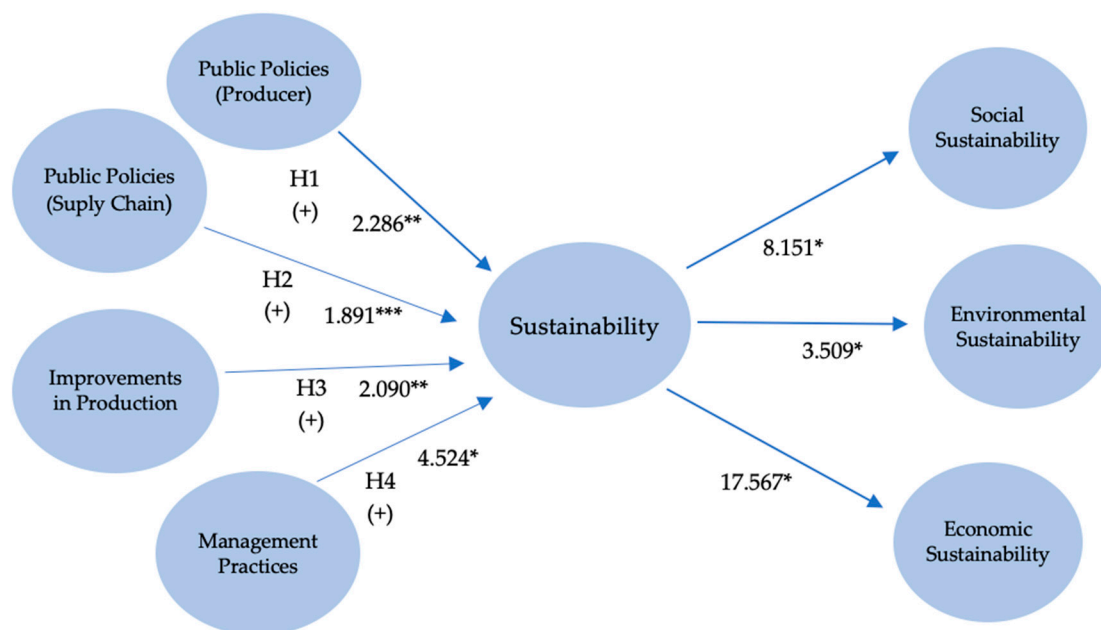
Figure 1. Second-order structural equation model. *** Significance level of 10%; ** Significance level of 5%; * Significance level of 1%. Source: research data.
