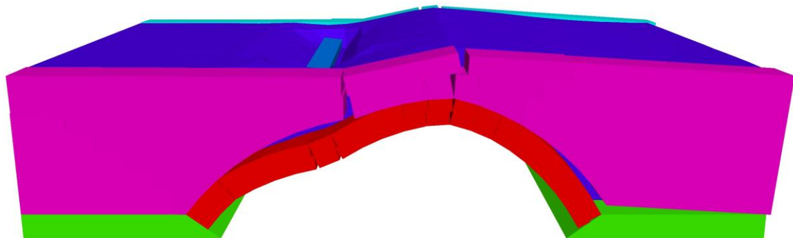
b) Plastic hinge formation near to the collapse
