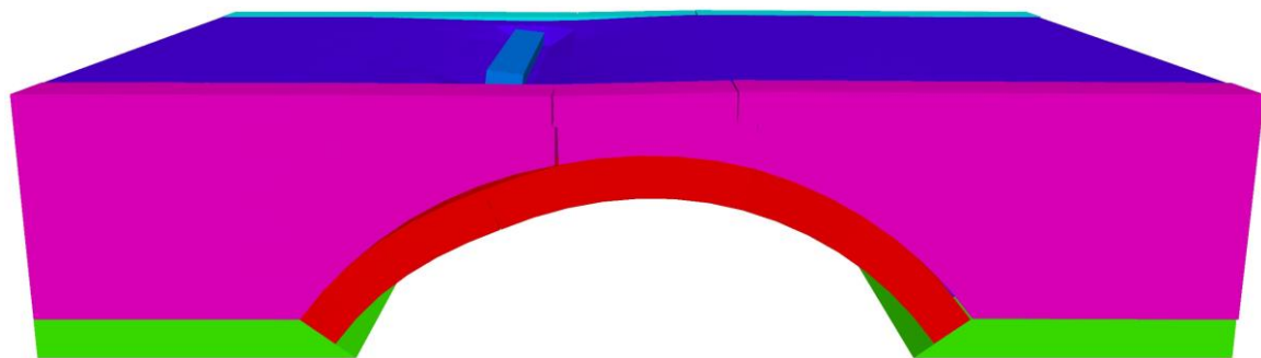
a) The spandrel wall detachment (260 kN)
