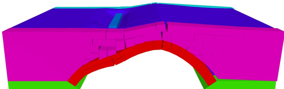
c) Ultimate damage state of the masonry arch bridge
