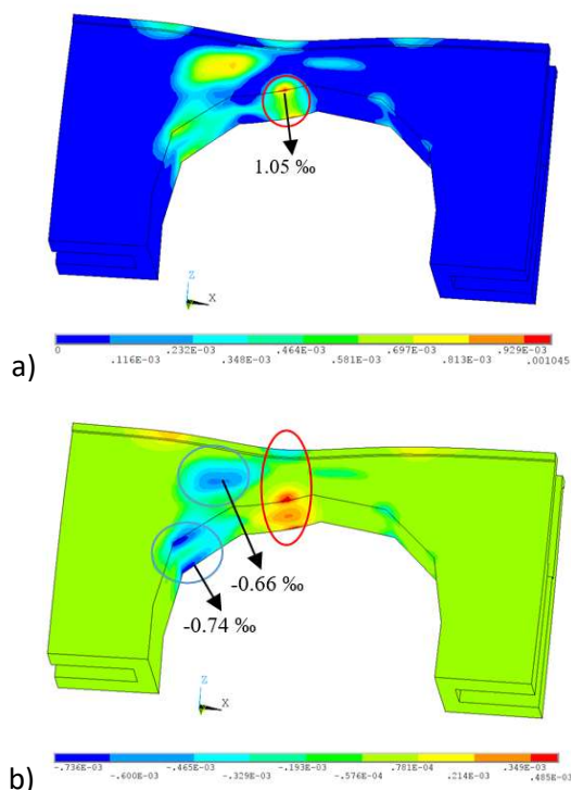
Figure 10. 3D sub-model of Leça bridge – plastic strain level for the final loading step (DL+10P): a) principal maximum strain and b) minimum plastic strain
