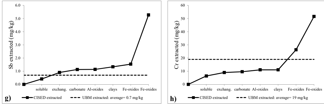
Figure 2. Median cumulative concentration in CISED extracted components (X-axis) and average bioaccessible concentration of Zn (a), Cd (b), Pb (c), Cu (d), Ni (e), Co (f) Sb (g), and Cr (h) (mg/kg) in sample group #1, #2 and #8. CISED extracted components are water soluble salt, exchangeable, Ca-carbonate, Al oxy-hydroxides, clays related, Fe oxy-hydroxides, and Fe-oxides.
