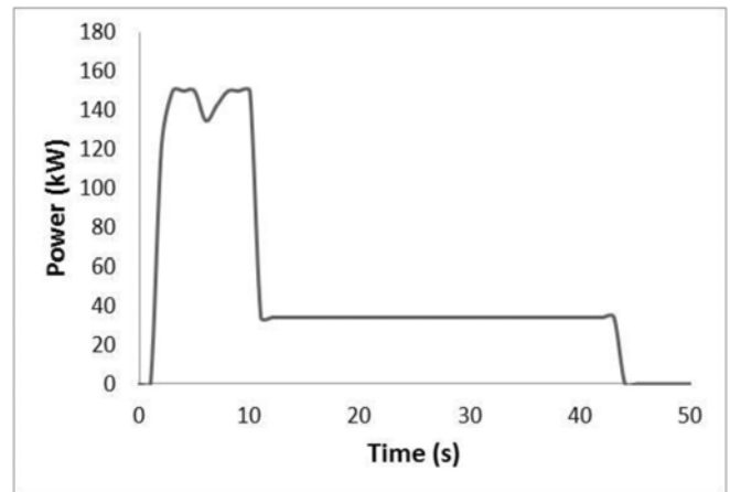
Figure 5. Power demand versus time
