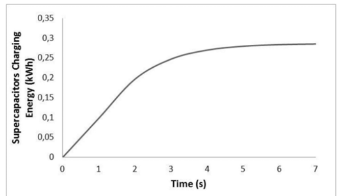
Figure 9. Supercapacitors absorbed energy versus time
