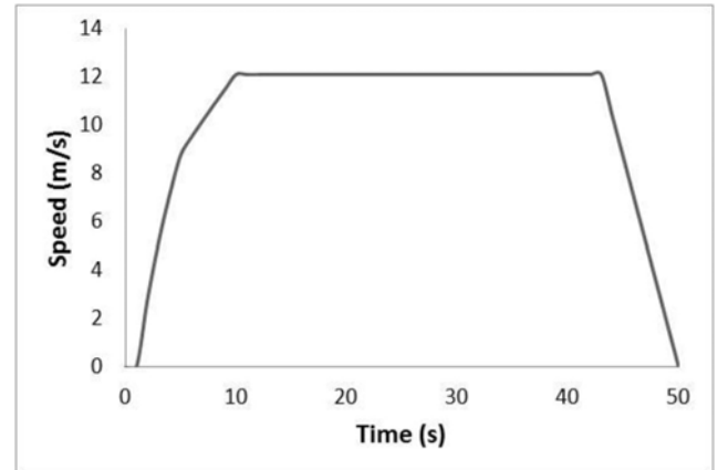
Figure 3. Driving cycle
