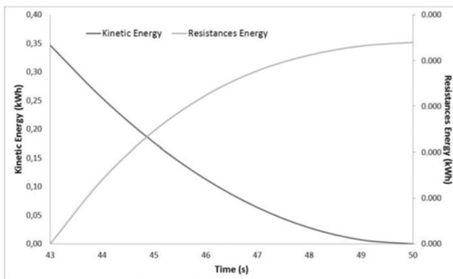
Figure 7. Kinetic Energy and Resistances Energy during braking versus time
