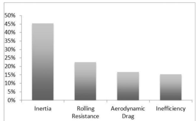
Figure 6. Energy Distribution
