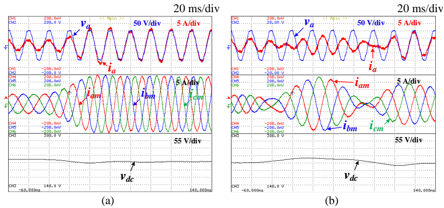
Fig. 10. Results obtained for the motor driving a 5 Nm load during: (a) Acceleration from 600 rpm to 800 rpm; (b) Deceleration from 800 rpm to 600 rpm.
