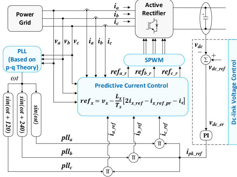
Fig. 2. Control diagram for the rectifier stage of the VSD.
