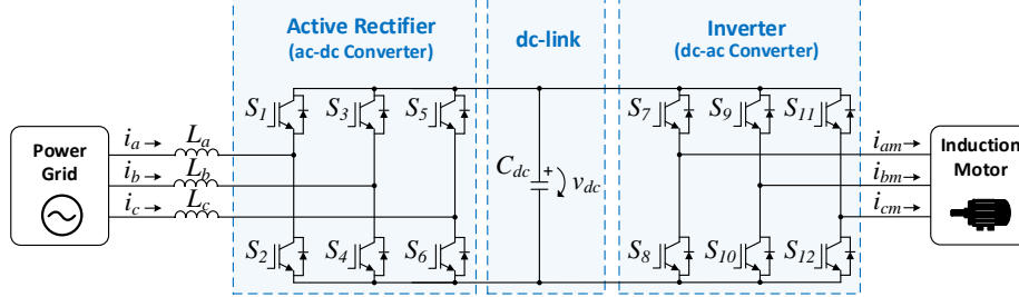
Fig. 1. Proposed system for the VSD.
