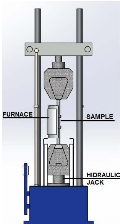
Fig. 2 Test setup for thermomechanical characterization of the bricks
