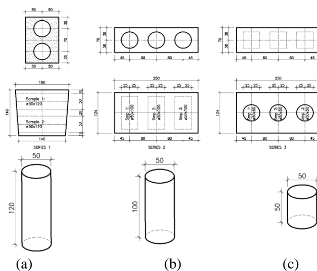
Fig. 1 Samples dimensions: (a) Series 1; (b) Series 2 and 4; (c) Serie 3
