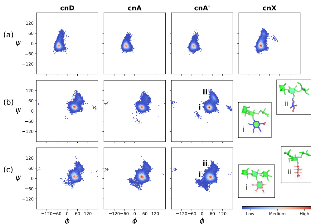
Figure 4. Heat maps of the glycosidic linkage orientation distribution over the last 400 ns of simulation in the two central RUs (RU3 and RU4) in the GXM chains. Row (a) shows the backbone \alpha DMAN(1 \rightarrow 3) \alpha DMAN linkage, row (b) the \beta DGlcA(1 \rightarrow 2) \alpha DMAN side chain linkage and row (c) the \beta DXyl(1 \rightarrow 2) \alpha DMAN side chain linkage. Glycosidic linkage orientations are shown as rotations of the linkage dihedral angles \phi and \psi . The insets in row (b) and (c) show the major face-on (i) and minor edge-on (ii) orientations of the \beta (1 \rightarrow 2)-linked side chains relative to the mannan backbone. The residues and substitutions are coloured as follows: \alpha DMan—green; \beta DGlcA—blue; \beta DXyl—pink; and 6-OAc—red.
