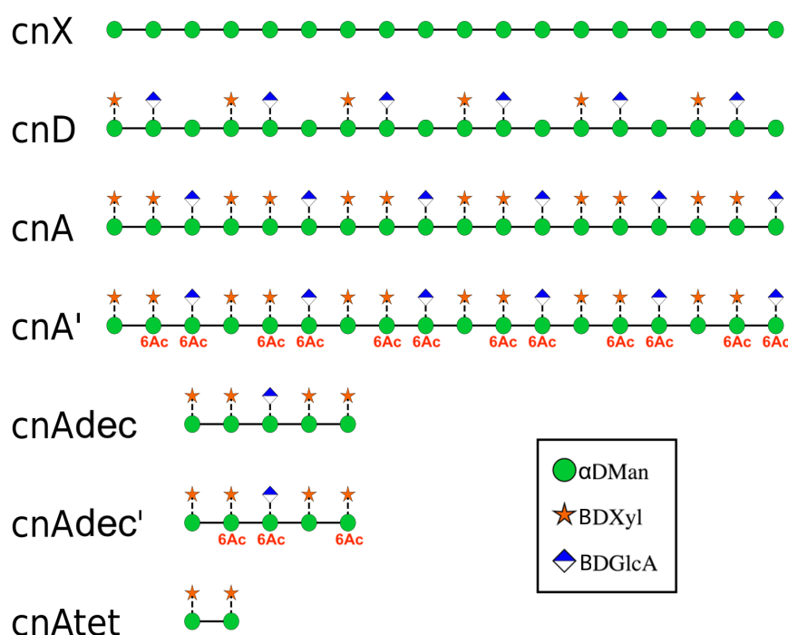
Figure 2. The array of GXM oligosaccharides simulated in this work, shown with the SNFG symbols [13,14] for the sugar residues. Six RUs of an unsubstituted backbone (cnX); the main repeat motifs in serogroup D (cnD) serogroup A (cnA) and 6-O-acetylated serogroup A (cnA') were run in separate simulations; and three shorter strands of serogroup A GXM: a decasaccharide (cnAdec), a 6-O-acetylated decasaccharide (cnAdec') and a tetrasaccharide (cnAtet).
