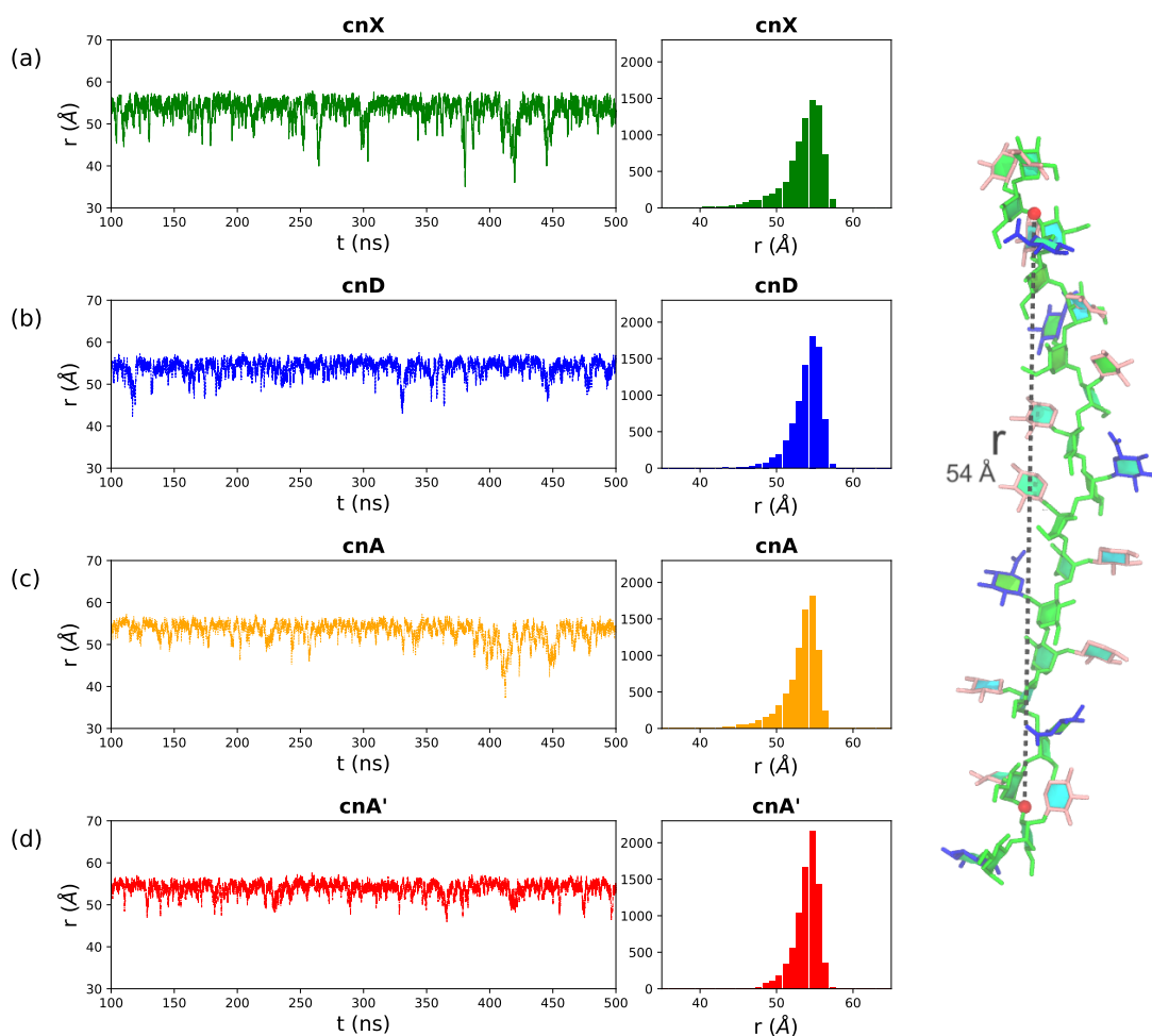
Figure 3. End-to-end distance, r , time series and corresponding histograms for the (a) cnX, (b) cnD, (c) cnA and (d) cnA' GXM chains. The first 100 ns of simulation are considered equilibration and are not shown. Here r is defined to exclude the two terminal residues on either end of the chain, as the distance from O3 in the second linkage to O3 in the 16th linkage in the 18-mannose backbone—labelled for cnA in the image on the right. The residues and substitutions are coloured as follows: \alpha DMan—green; \beta DGlcA—blue; \beta DXyl—pink; and 6-OAc—red.
