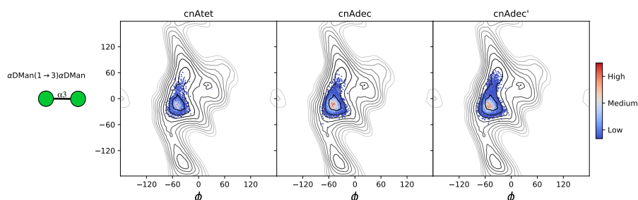
Figure A2. Heat maps of the distribution of the central backbone \alpha DMan(1 \rightarrow 3) \alpha DMan glycosidic linkage orientation for a the cnAtet tetrasaccharide fragment ( left ) and deca-saccharide cnAdec ( middle ) as well as a 6-O-acetylated deca-saccharide cnAdec' ( right ). Glycosidic linkage orientations are shown as rotations of the linkage dihedral angles \phi and \psi .
