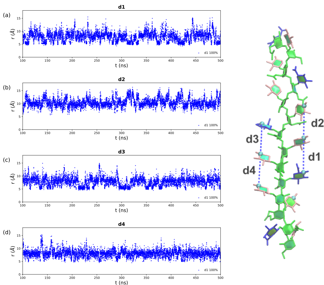
Figure A4. The time series for the distances between interacting side chains in the cnA' molecule labeled on the right. (a) The \beta DGlcA and \beta DXyl distance d1, (b) the \beta DXyl and \beta DXyl distance d2 (c) the \beta DGlcA and \beta DXyl distance d3 and (d) the \beta DXyl and \beta DXyl distance d4. Here in each case d is defined to as the distance from C4 in one residue to C4 in the proximal side chain residue. The first 100 ns of simulation are considered equilibration and are not shown. The residues and substitutions are coloured as follows: \alpha DMan—green; \beta DGlcA—blue; \beta DXyl—pink and 6-OAc—red.
