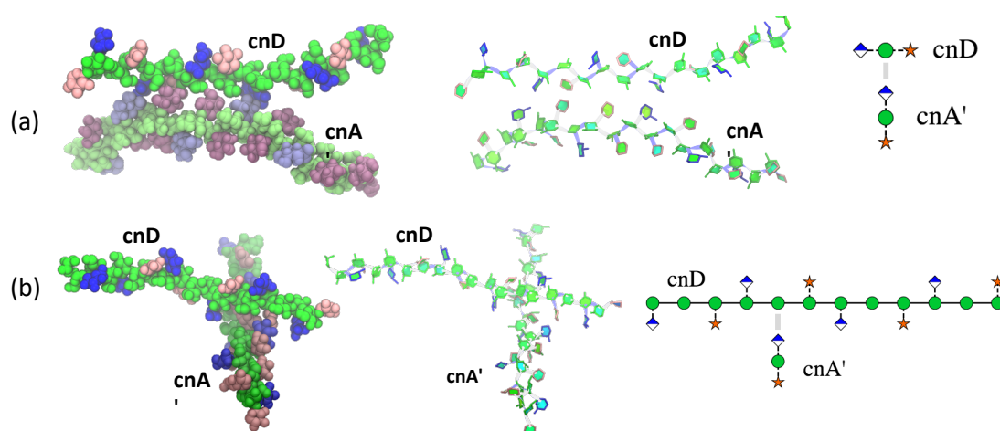
Figure 6. Examples of self-aggregation interactions between 6-RU strands of cnD and cnA in (a) parallel and (b) orthogonal arrangements. Molecules are depicted using the VMD [26] van der Waals representation (left); and the VMD PaperChain and Twister representations (middle) and a schematic (right). The saccharide residues are coloured as follows: \alpha DMan—green; \beta DGlcA—blue; \beta DXyl—pink; and 6-OAc—red.
