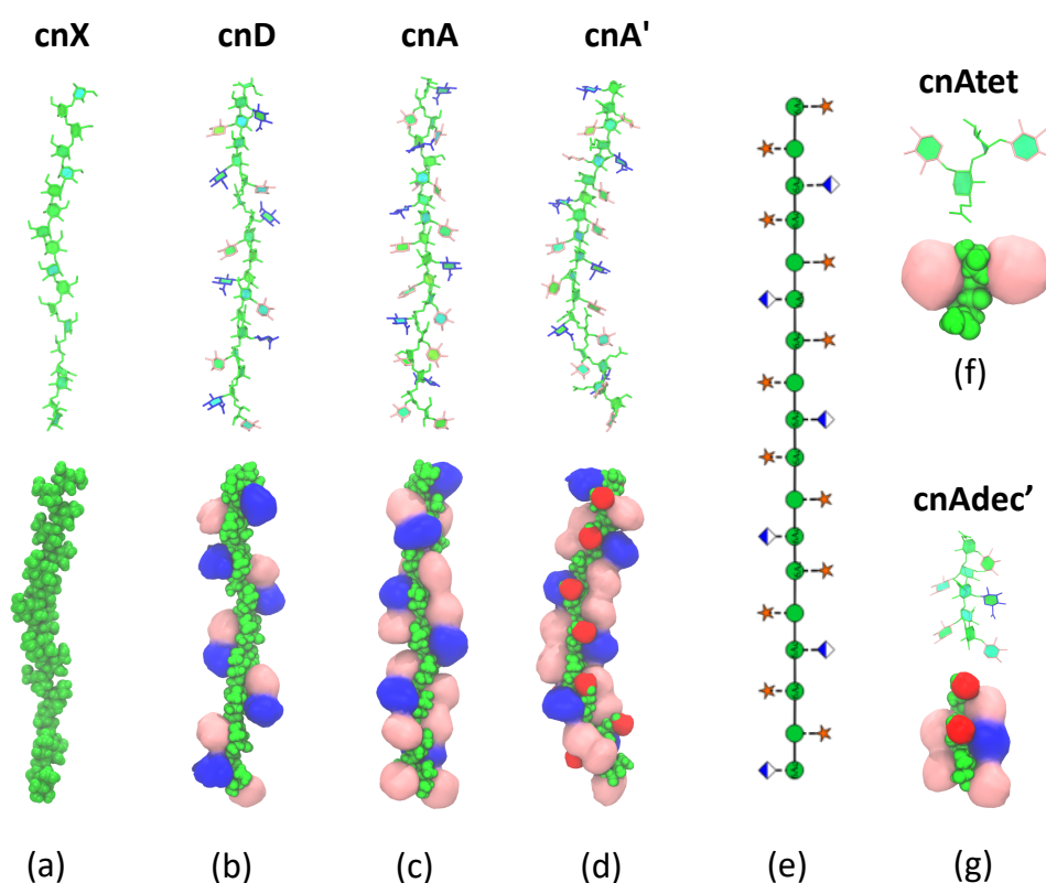
Figure 5. Dominant conformations of the GXM molecules shown with two representations in the VDM package [26]—the PaperChain visualisation [27] to highlight the conformation of the backbone and space-filling representations to highlight the exposed binding surface. Representative conformations are shown for (a) the unsubstituted mannan backbone cnX ; (b) cnD ; (c) cnA ; (d) and cnA' (6- O -acetylated). A schematic for the arrangement of the side chain substitutions is shown in (e) using the SNFG symbols for the sugar residues [13,14]. Representative conformations of the chain fragments are shown for the tetrasaccharide (f) cnAtet and the 6- O -acetylated decasaccharide (g) cnAdec' . The chain substitutions in all representations are coloured as follows: \alpha DMAN—green; \beta DGlcA—blue; \beta DXyl—pink and 6-OAc—red.
