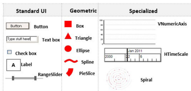
FIGURE 2. Examples of visual objects that Uvis supports.
