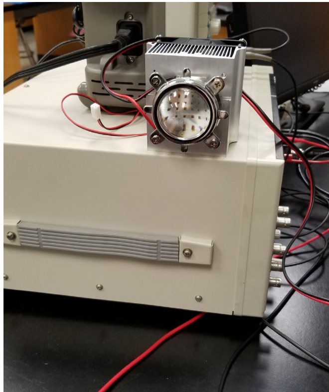
Figure 20. High-power Red LED with Heat Sink and Focusing Lens
