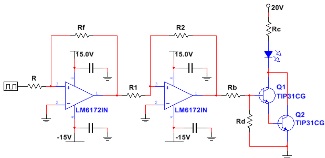
Figure 3. LED Driver Circuit
