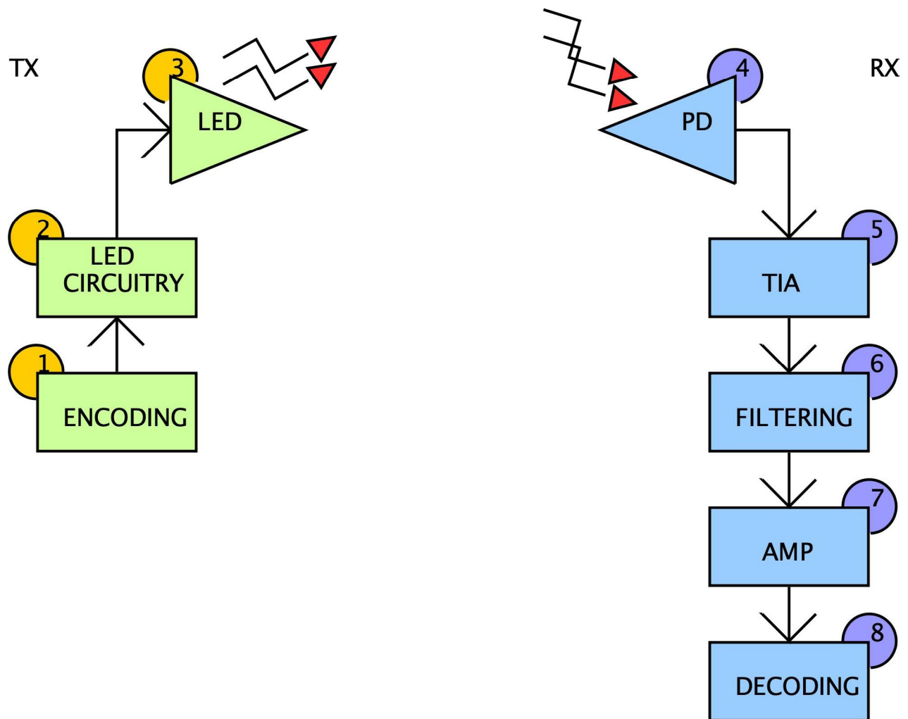
Figure 2. Block Diagram of VLC System
