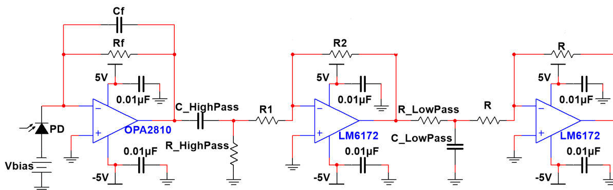
Figure 4. Photodiode Receiver Circuit
