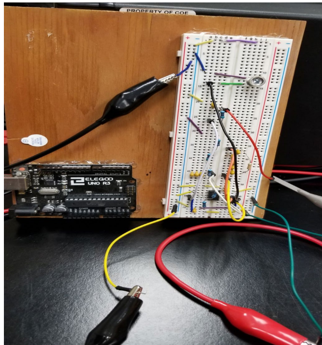
Figure 21. Receiver Circuit Design on Breadboard
