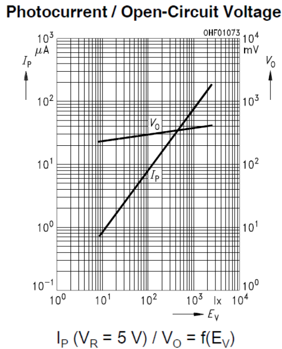
Figure 7. BPX61 Photodiode Photocurrent and Open-circuit Voltage as a Function of Luminosity
