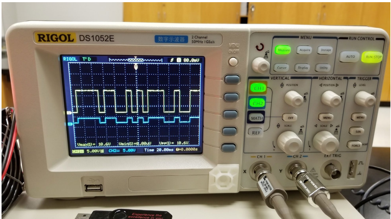
Figure 23. Transmitter and Receiver Voltage Analysis on the Oscilloscope
