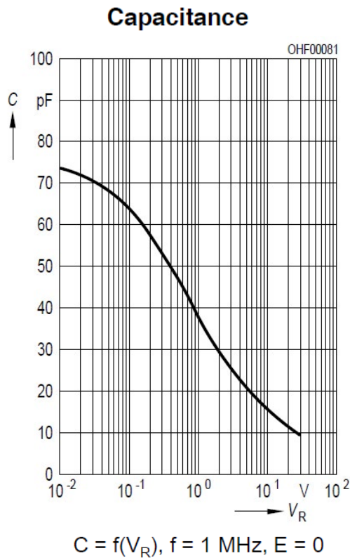
Figure 6. BPX61 Photodiode Junction Capacitance as a Function of Reverse Bias Voltage
