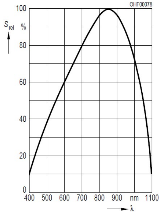
Figure 5. BPX61 Photodiode Relative Spectral Sensitivity as a Function of Wavelength
