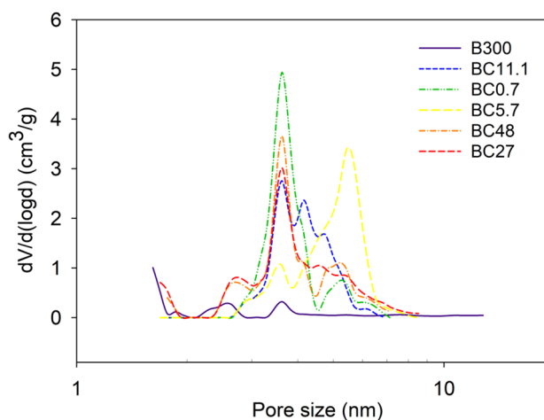
Fig. 4 Pore size distribution of the catalysts
