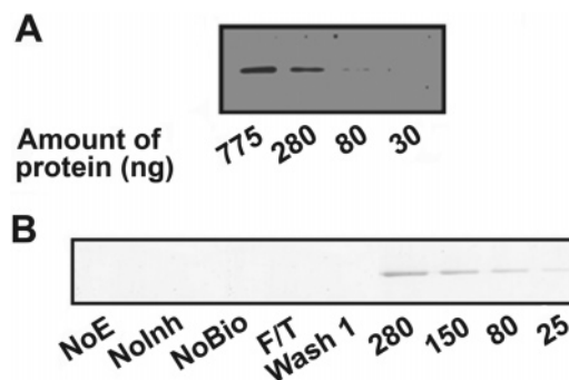
Figure 4. (A) Western blot showing the detection limit of 1, used in conjunction with Staudinger ligation: amounts of VCNagZ were 775, 280, 80, 30 ng. (B) SYPRO-stained 10% SDS-PAGE showing the detection limit of 1, used in conjunction with copper-catalyzed Sharpless-Meldal click reaction. Lanes shown (left to right); no enzyme, no inhibitor 1, no biotin label, flow through, wash 1, 280 ng of VCNagZ, 150 ng of VCNagZ, 80 ng VCNagZ, 25 ng VCNagZ.
