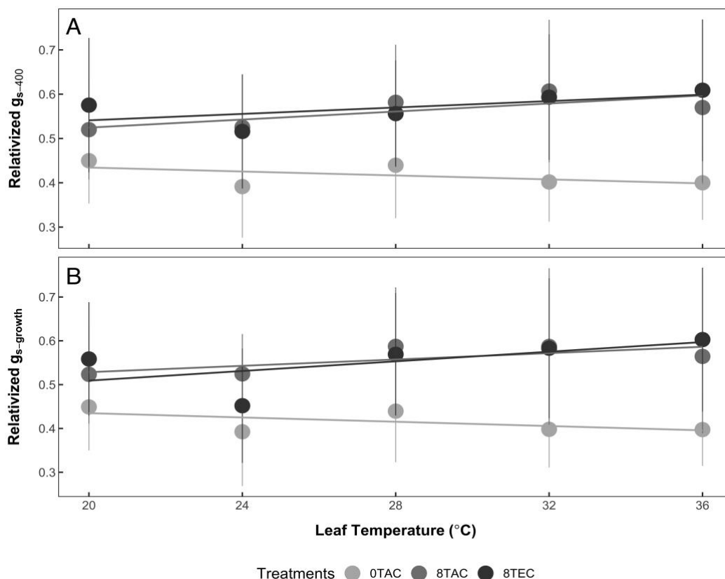
Figure 3.5. Relativized stomatal conductance of temperature curves. Stomatal conductance was measured at: A) a common CO 2 of 400 ppm ( g_{s-400} ) and B) growth CO 2 ( g_{s-growth} ). Curves were relativized by the maximum rate of stomatal conductance per replicate. Points represent means \pm SE; n = 6 . Light grey, ambient temperature with ambient CO 2 (0TAC); medium grey, +8 °C warming with AC (8TAC); dark grey, 8T with elevated CO 2 (8TEC).
