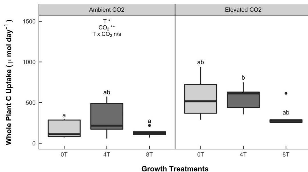
Figure 2.8. Whole plant daily C uptake of seedlings across the growth treatments.
