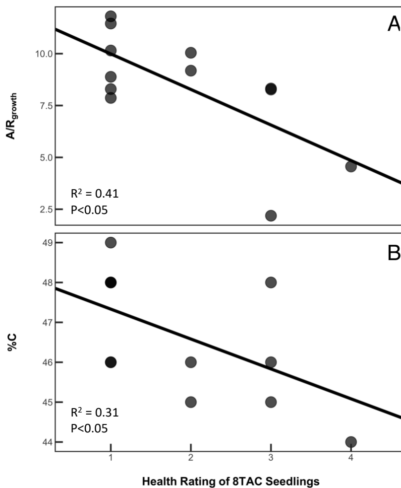
Figure 2.11. Relationship between seedling health rating and leaf C balance and foliar C. A) The ratio of net CO 2 assimilation rate to shoot dark respiration rate at growth conditions ( A/R_{\text{growth}} ) and B) the percent needle carbon (%C). Points represent individual seedlings, n = 12 . Solid line, linear regression.
