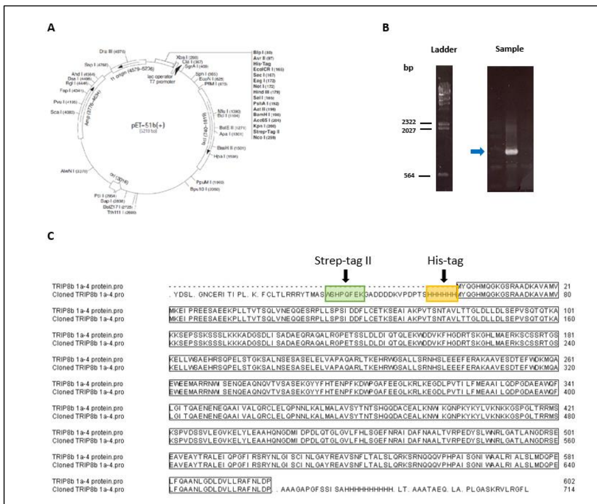
Figure 3.1 Cloning TRIP8b(1a-4) into pET51b+ plasmid.
