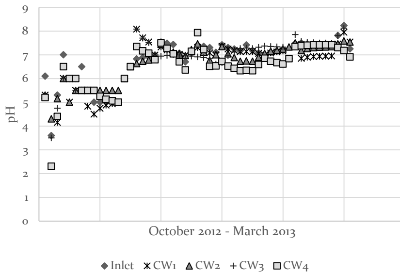
Figure 3: Temporal pH variation (October 2012- March 2013) from inlet and outlet on each constructed wetland (n= 50 per location).
