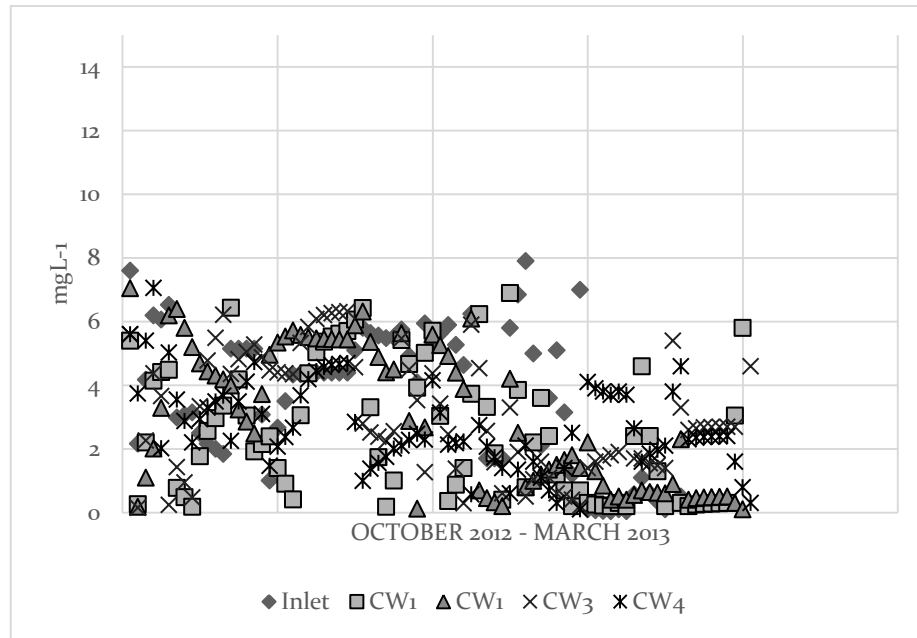
Figure 4: Temporal dissolved oxygen variation (October 2012-March 2013) from inlet and output on each constructed wetland (n= 80-85 per location).
