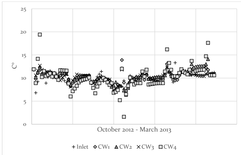
Figure 2. Temporal temperature (C°) variation (October 2012-March 2013) from inlet and output on each constructed wetland (n= 80-90 per location).
