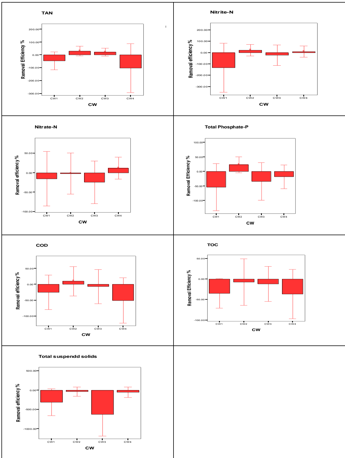
Figure 5. Comparison of removal efficiency for several chemical and physical pollutants in four constructed wetlands during the sampling season (October 2012-March 2013). Boxes represent mean and standard error; n=20-25 per location.
