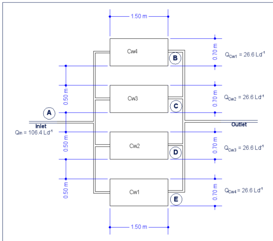
Figure 1: Connection to the RAS, Constructed wetland distribution and caudal in each wetland system.
