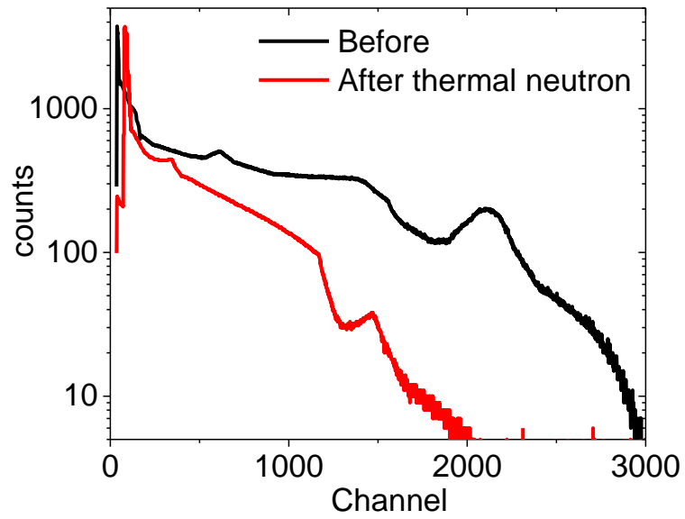
Supplementary Figure 11. Pulse height spectra of ^{137}\text{Cs} measured before and after thermal neutron exposure of 4.8 MeV. The light yield drops from 10,500 to 7,000 ph per MeV after thermal neutron measurement while the energy resolution increases from 17.6 to 25.9.
