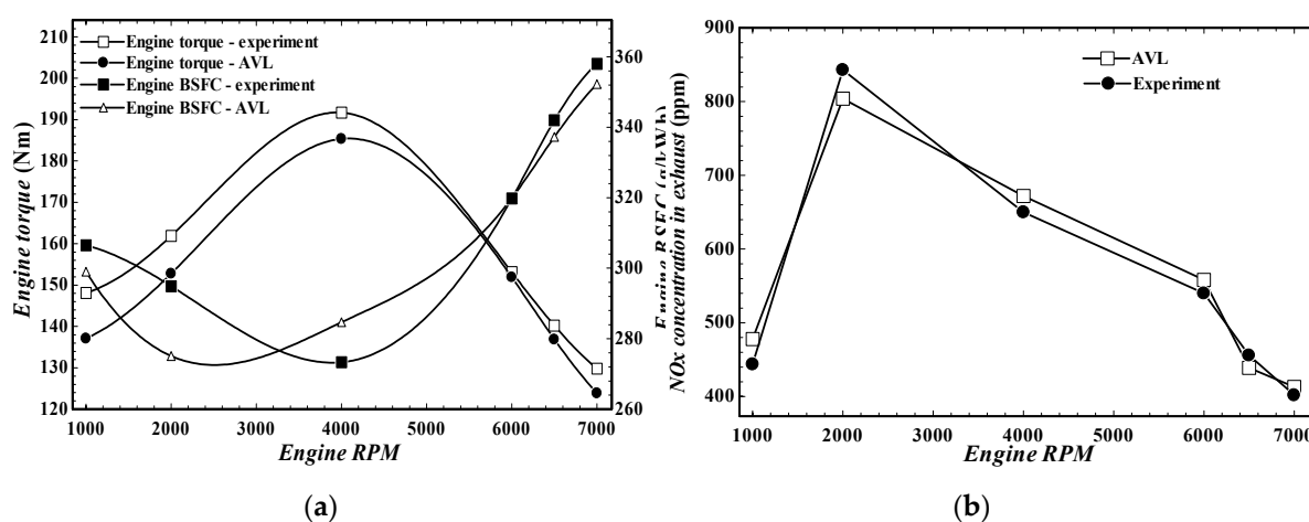
Figure 3. (a) Engine Torque and BSFC and (b) NOx concentration in the exhaust in the AVL model and experimental tests obtained from running the engine by gasoline at full load and various RPMs.
