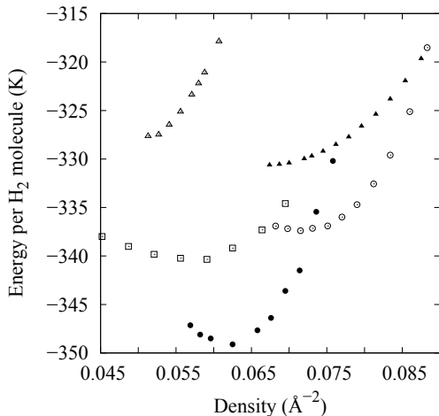
FIG. 2. Energies per \text{H}_2 molecule for different adsorbed phases on a (5,5) tube. We display here the liquid (open squares), the different incommensurate solids: five-in-a-row (solid circles), six-in-a row (open circles), four-in-a-row (open triangles) and seven-in-a-row (full triangles).
