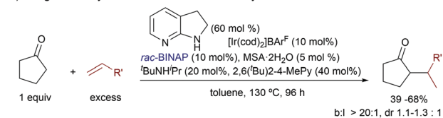
Scheme 21 Ir-Catalyzed branched-selective ketone \alpha -alkylation by Dong and co-workers.
