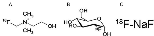
FIGURE 1. Chemical structure of (A) ^{18}\text{F} -Choline, (B) ^{18}\text{F} -FDG, and (C) ^{18}\text{F} -NaF.
