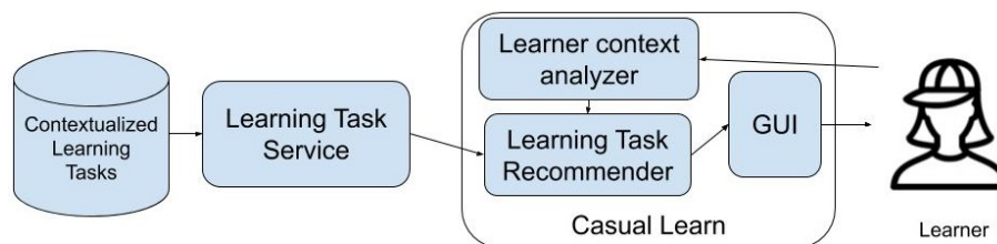
Fig. 1. Software architecture of CasualLearn. Details about Contextualized Learning Tasks and Learning Task Service can be found at [3].
