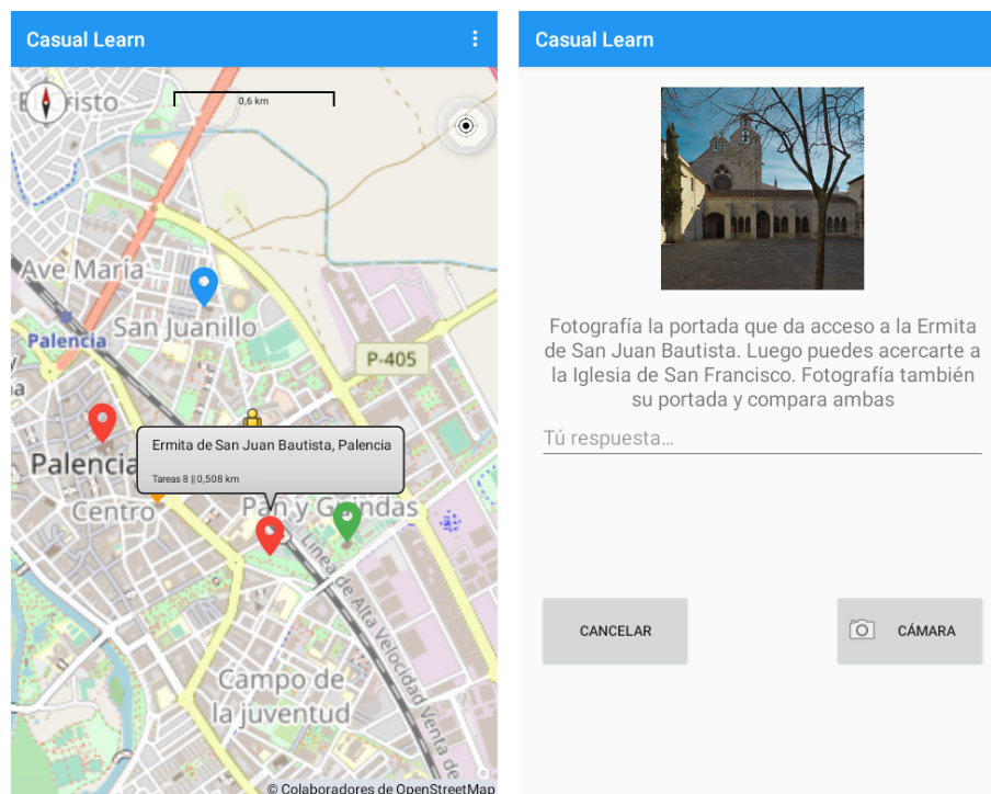
Fig. 2. CasualLearn GUI snapshots: map view interface (left) and task interface (right). The text in the task interface says: "Take a photo of the portal of the Hermitage of Saint John. Then, you can go to the Church of Saint Francis. Take another photograph of its portal and compare both of them."
