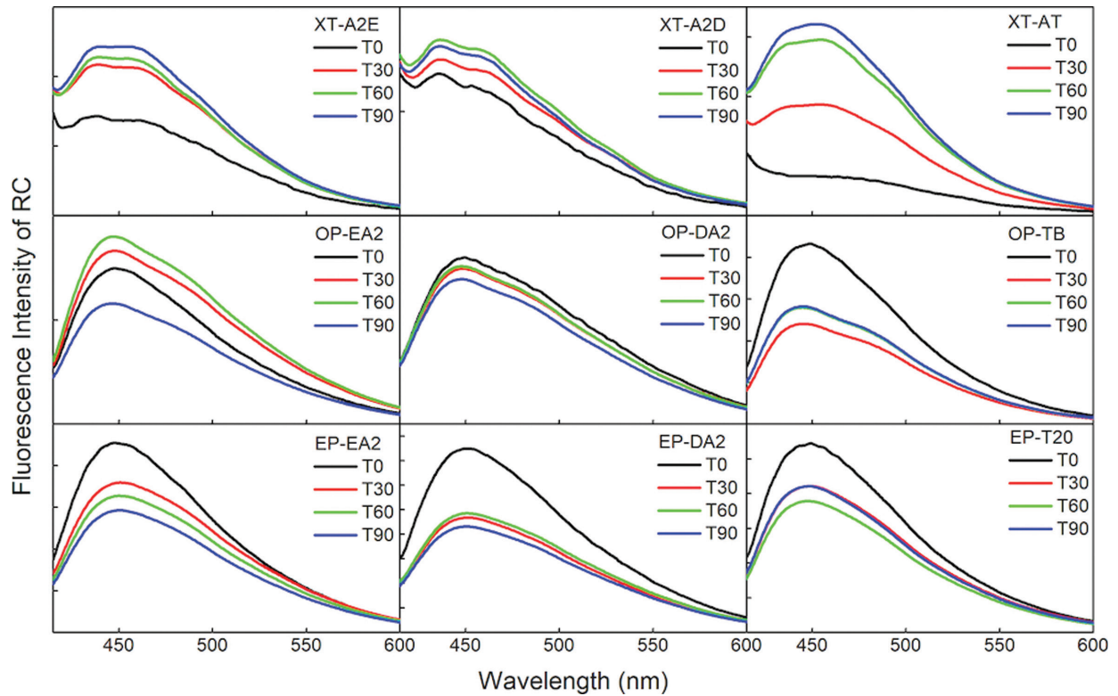
Fig. 3: Spectras of fluorescence intensity variations of composite resins in different times: baseline (T0), after 30 days (T30), after 60 days (T60) and after 90 days (T90).
