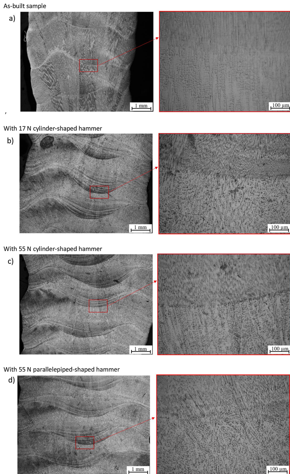
Fig. 9. (a) Micrographs of the as-built, (b) hot-forged with 17 N cylinder-shaped hammer, (c) hot-forged with 55 N cylinder-shaped hammer, (d) hot-forged with 55 N parallelepiped-shaped hammer.
