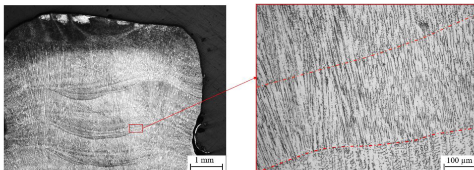
Fig. 12. Micrograph showing grain growth discontinuities (dash lines) in the hot-forged samples.
