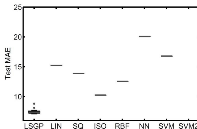
Figure 5. Boxplots of the test MAE calculated over 100 runs. On each box, the central mark is the median, the edges of the box are the 25th and 75th percentiles, and the whiskers extend to the most extreme data points not considered outliers. The MAE is expressed in Euros. LIN stands for linear regression, SQ stands for ordinary least square regression, ISO stands for isotonic regression, RBF stands for radial basis function network, NN stands for multilayer perceptron trained with backpropagation, and SVM stands for support vector machine with a polynomial kernel (of second degree for SVM2).
