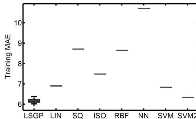
Figure 4. Boxplots of the training MAE calculated over 100 runs. On each box, the central mark is the median, the edges of the box are the 25th and 75th percentiles, and the whiskers extend to the most extreme data points not considered outliers. The MAE is expressed in Euros. LIN stands for linear regression, SQ stands for ordinary least square regression, ISO stands for isotonic regression, RBF stands for radial basis function network, NN stands for multilayer perceptron trained with backpropagation, and SVM stands for support vector machine with a polynomial kernel (of second degree for SVM2).
