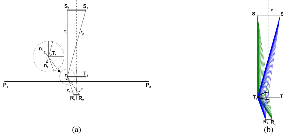
FIGURE 4. To The RR SMS optic design process. (a) Definition of the normals \mathbf{n}_1 and \mathbf{n}_2 (b) the RR SMS chains.
