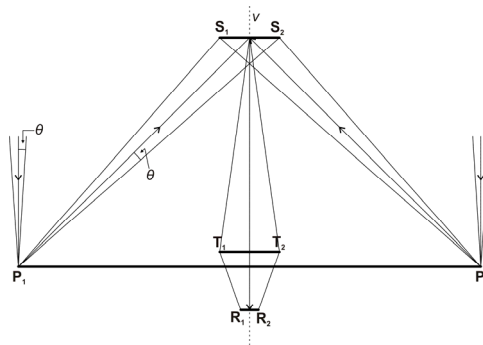
FIGURE 1. Schematic representation of the Cassegrainian approach.
