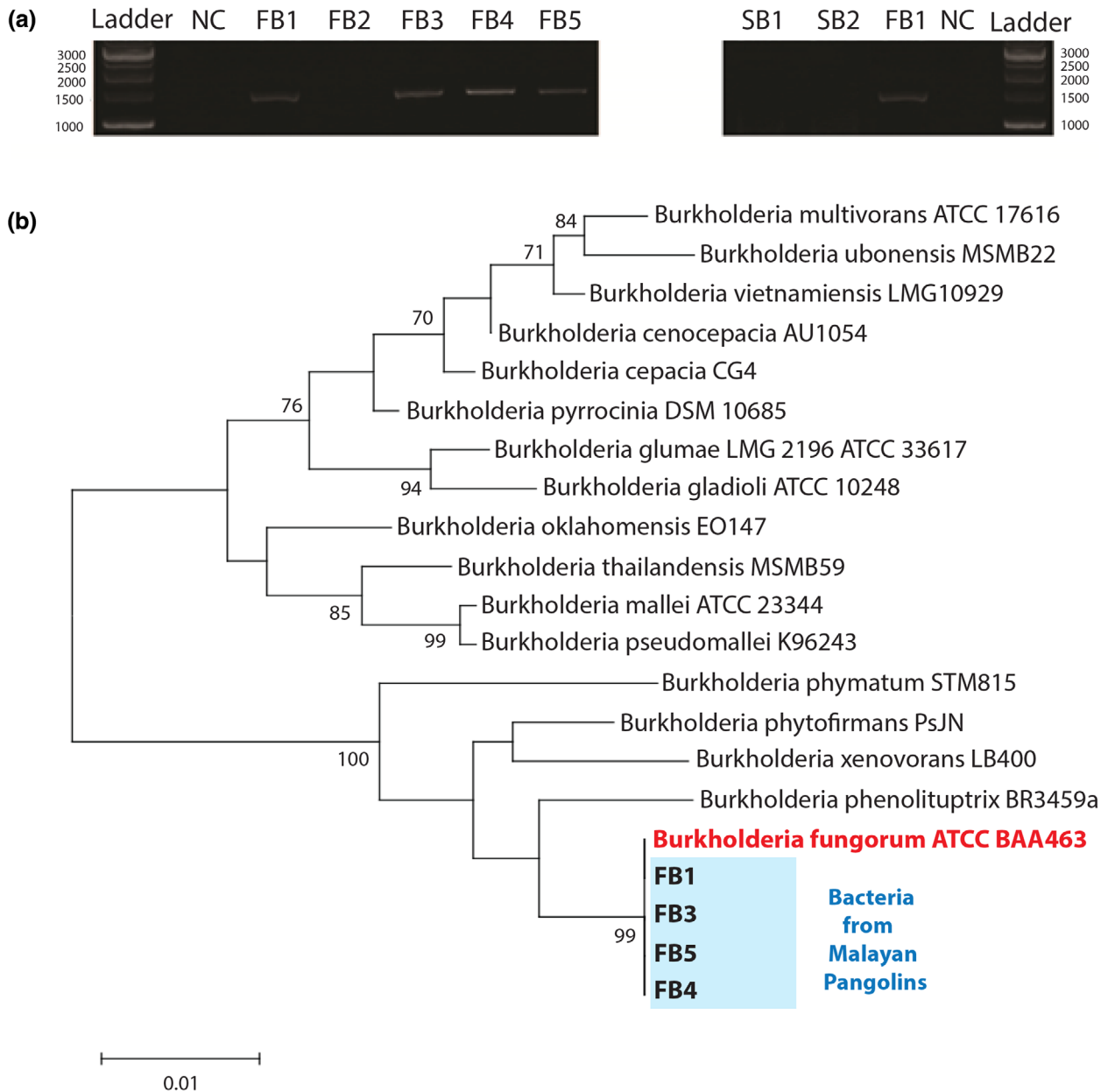
FIGURE 4 Identification of Burkholderia fungorum in Malayan pangolins. (a) PCR assays using the blood of seven pangolin individuals from two independent batches (Batch 1: FB1-5; Batch 2: SB1-2). Using the universal 16S gene primers to identify the presence of bacteria in all pangolin samples. NC (without DNA) is the negative control. (b) PCR products were sequenced using Sanger sequencing. The phylogenetic tree was generated using the 16S gene sequences and the maximum likelihood method. Bootstrap numbers were generated in 1,000 replicates. Nodes with bootstrap support values of 70 or greater are indicated
