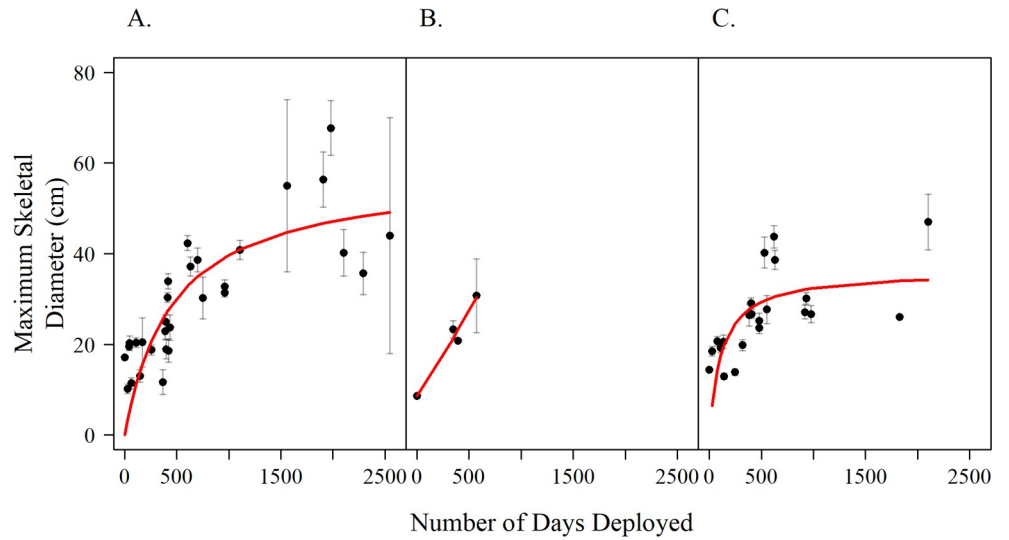
Fig 6. Maximum skeletal diameter of A. cervicornis colonies over time by habitat type. A) spur-and-groove, B) patch-reef, and C) hardbottom. Dots represent sample dates. Error bars represent standard error. Trendlines are Gompertz growth functions.
