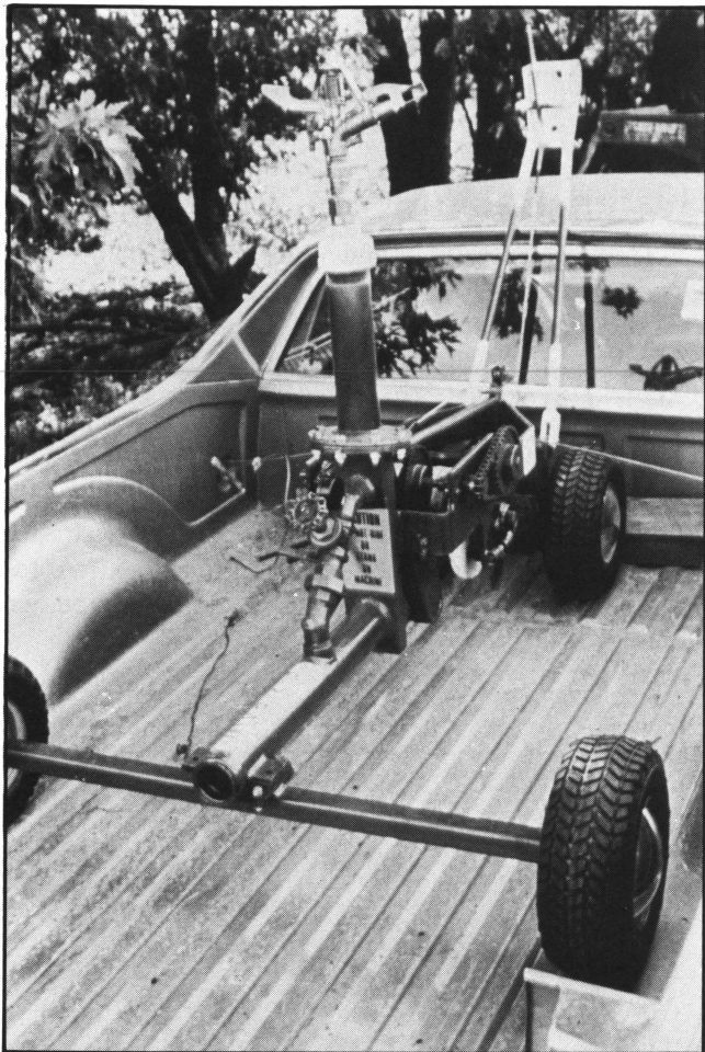
Figure 9. A small traveling gun may reduce labor requirements at a cost compatible with the production facility.
