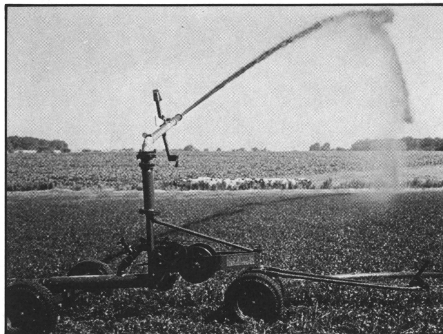
Figure 7. Conventional traveling guns provide excellent distribution of lagoon effluent.
