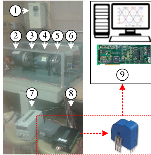
Fig. 6.8. Experimental setup: (1) power source and VFD, (2) IM under test, (3) coupling, (4) speed-reduction gearbox, (5) magnetic clutch, (7) DC power source, (8) current transformers and signal conditioning apparatus, (9) conventional DAQ board and computing device.
