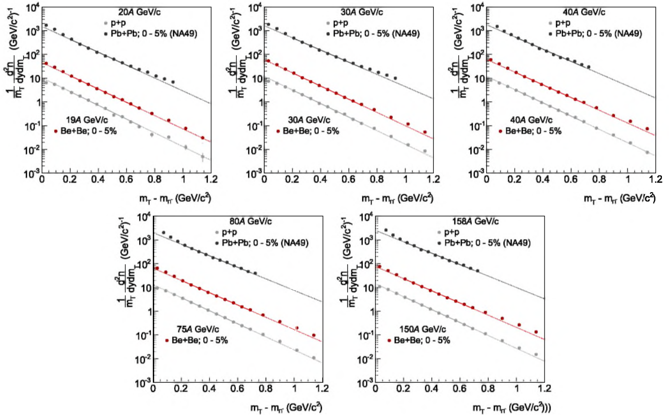
Fig. 13 Transverse mass spectra \frac{1}{m_T} \frac{d^2n}{dy dm_T} of negatively charged pions produced in central Be + Be collisions at the SPS energies. Statis-
