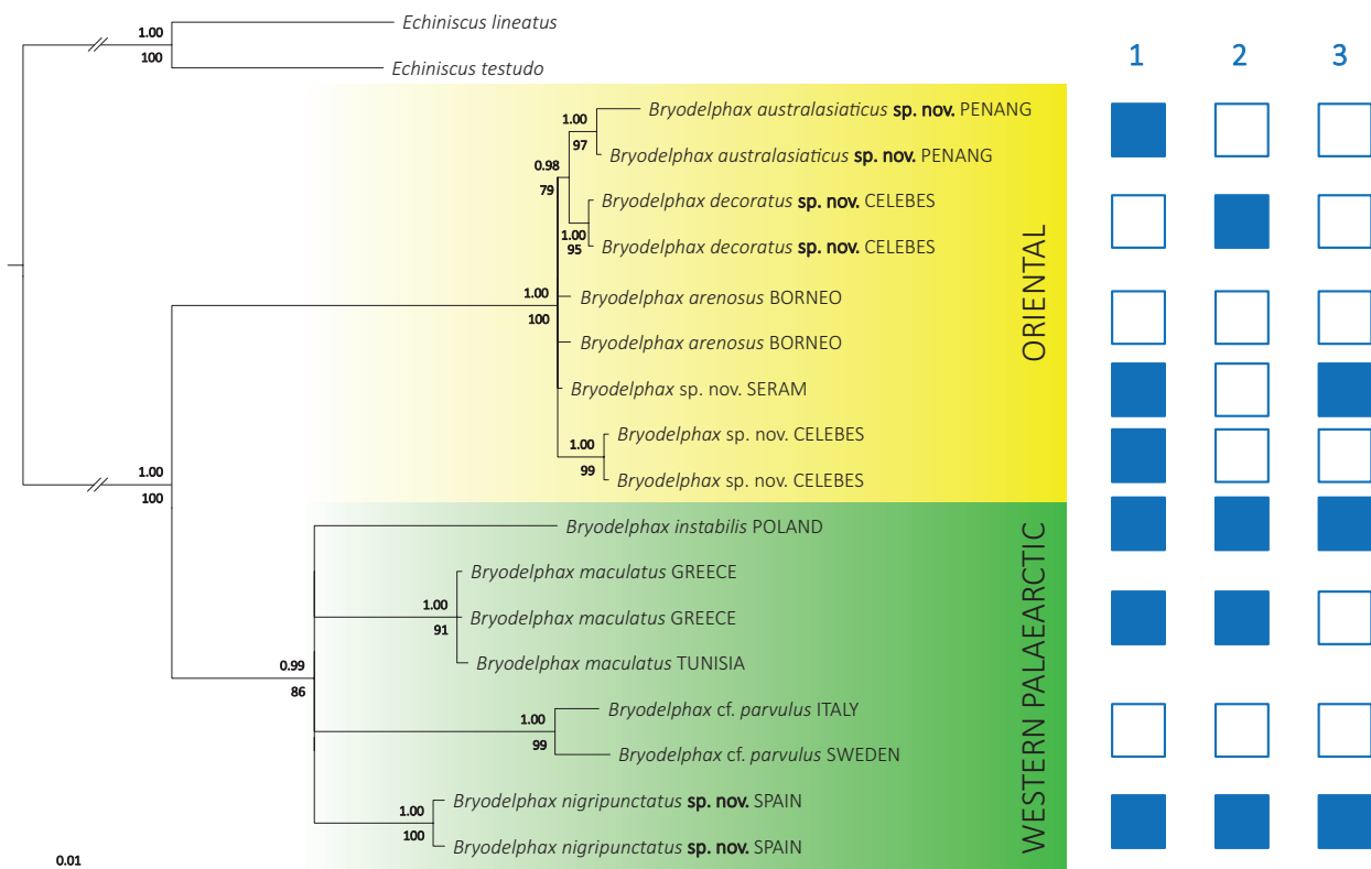
Figure 1. BI and ML concatenated (18S rRNA + 28S rRNA) phylogenetic tree of Bryodelphax Thulin, 1928; Echiniscus spp. were used as outgroup taxa. Bayesian posterior probability values ( \geq 0.90 ) are given above tree branches, whereas ML bootstrap support values ( \geq 70 ) are below branches. The scale bar represents 0.01 substitutions/site in the Bayesian tree. Trait mapping (blue square – presence, empty square – absence): 1 – ventral plates; 2 – granules on dorsal plates; 3 – males in population.
