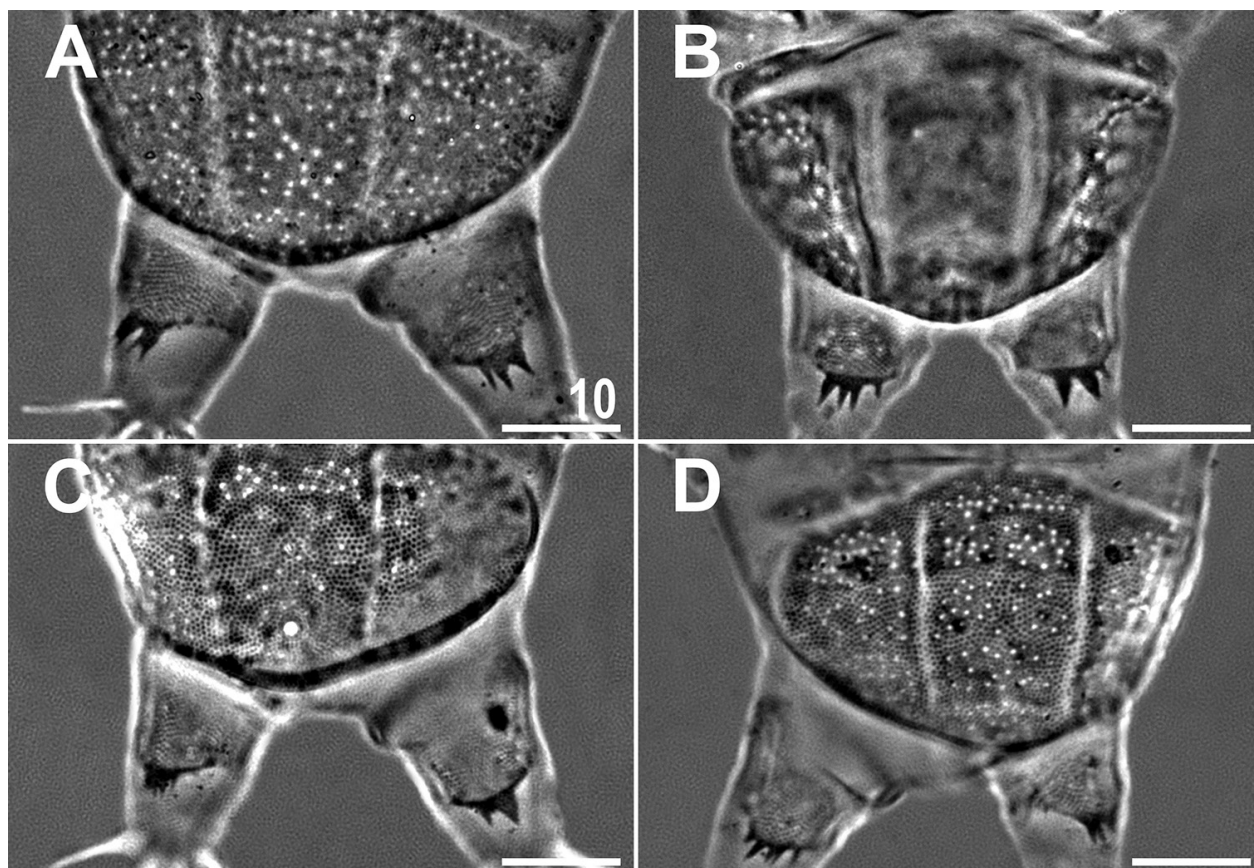
Figure 11. Variability of the dentate collar IV in Bryodelphax nigripunctatus sp. nov. (paratypes, PCM). Scale bars: 10 \mu\text{m} .
