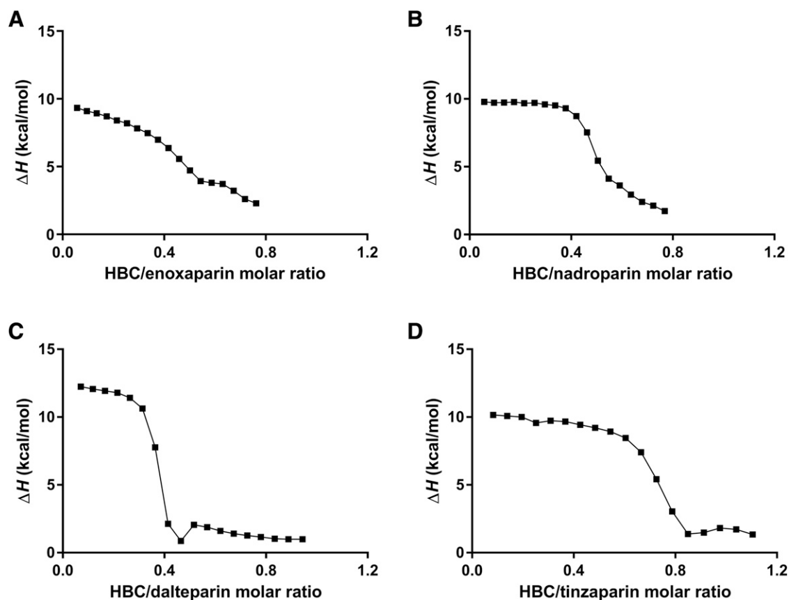
Fig. 4. Estimated heat of binding for the titration of HBC into enoxaparin (A), nadroparin (B), dalteparin (C), and tinzaparin (D).
