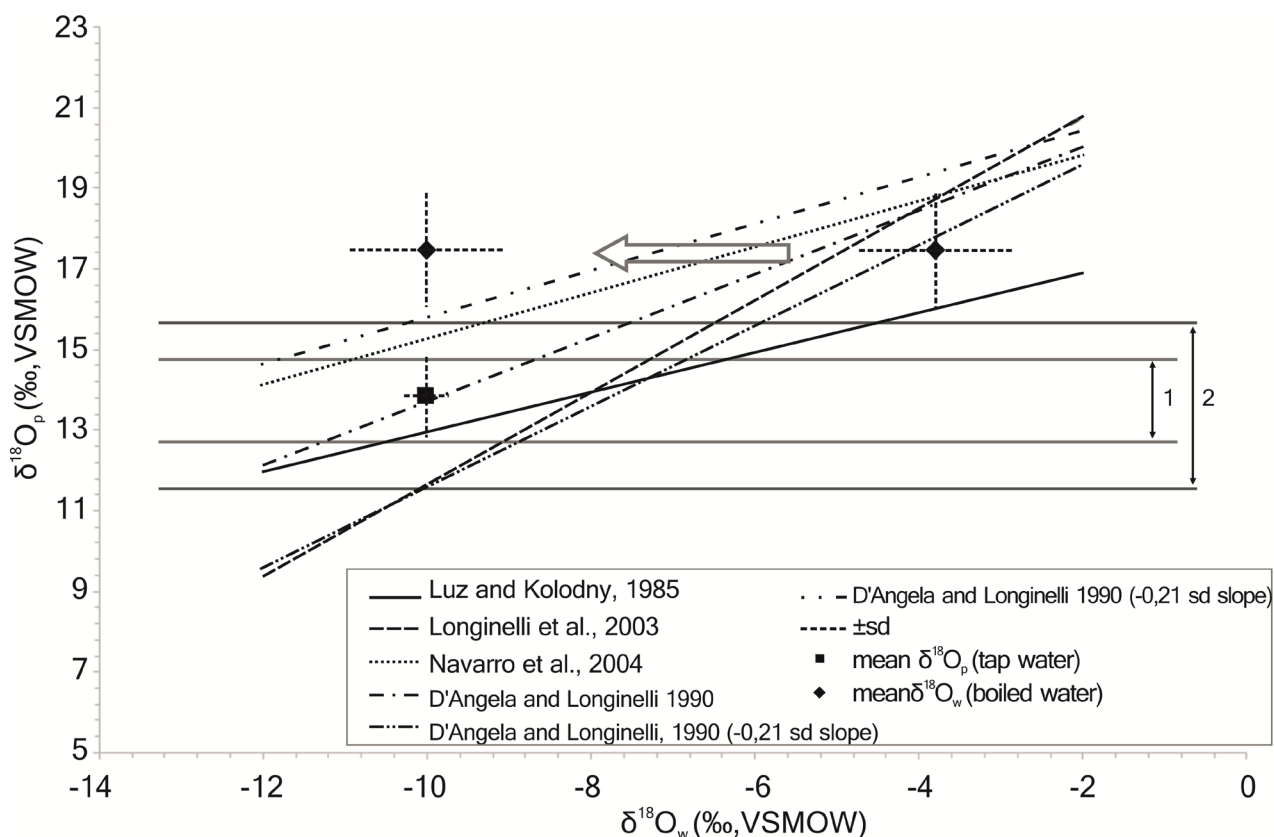
Fig. 4. \delta^{18}\text{O}_p mean values ( \pm sd) of bone samples from rats drinking tap water (square) and thermally processed water (diamond) plotted versus the \delta^{18}\text{O} average of tap water ( -10.011\text{‰} ) and thermally processed water ( -3.7894\text{‰} ) respectively. Horizontal lines determine the range of \delta^{18}\text{O} variability in the environmental water from the area of Kraków. Scope no. 1 was determined based on the results obtained for rats drinking tap water \pm 1 sd. Scope no. 2 was determined as the minimum and maximum values determined on the basis of the presented regression lines. The results obtained for rats drinking boiled water were shifted to the same level as the results for rats drinking tap water to better visualize the relationship to the compared groups and reference to ranges showing the local environmental level.
