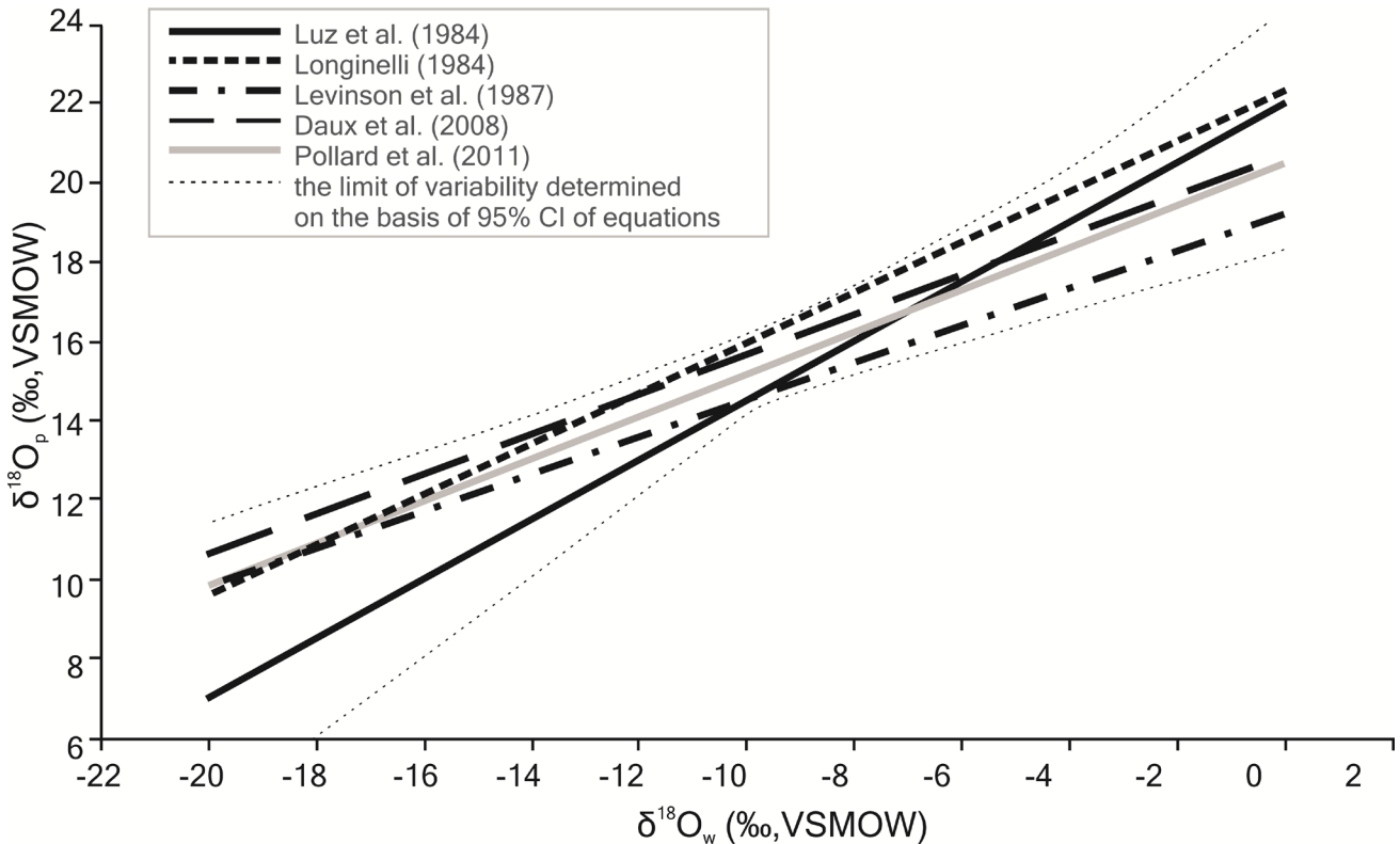
Fig. 5. Variability of oxygen isotopic composition based on the relationship between \delta^{18}\text{O}_p and \delta^{18}\text{O}_w in human studies.
