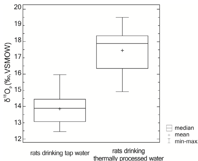
Fig. 3. The difference in the values of isotopic delta of bone phosphates in animals consuming two different types of water.
