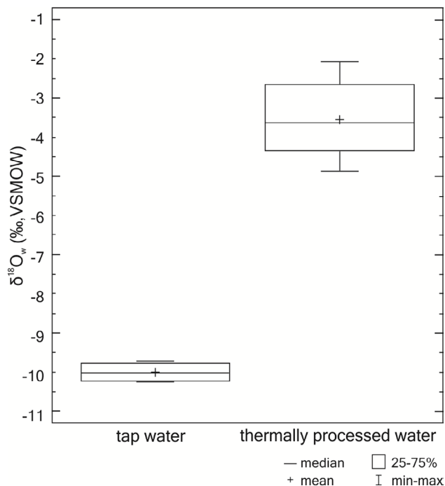
Fig. 1. The values of oxygen isotopic delta of tap water and thermally processed water with the measurement errors.
