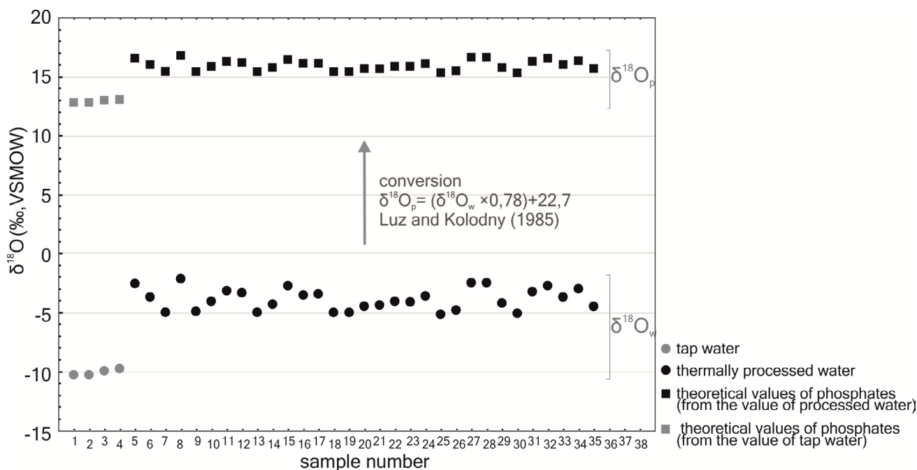
Fig. 2. The isotopic composition of water given to laboratory rats, recalculated to values of the isotopic composition of apatite phosphates in specimens potentially consuming water with a certain composition.
