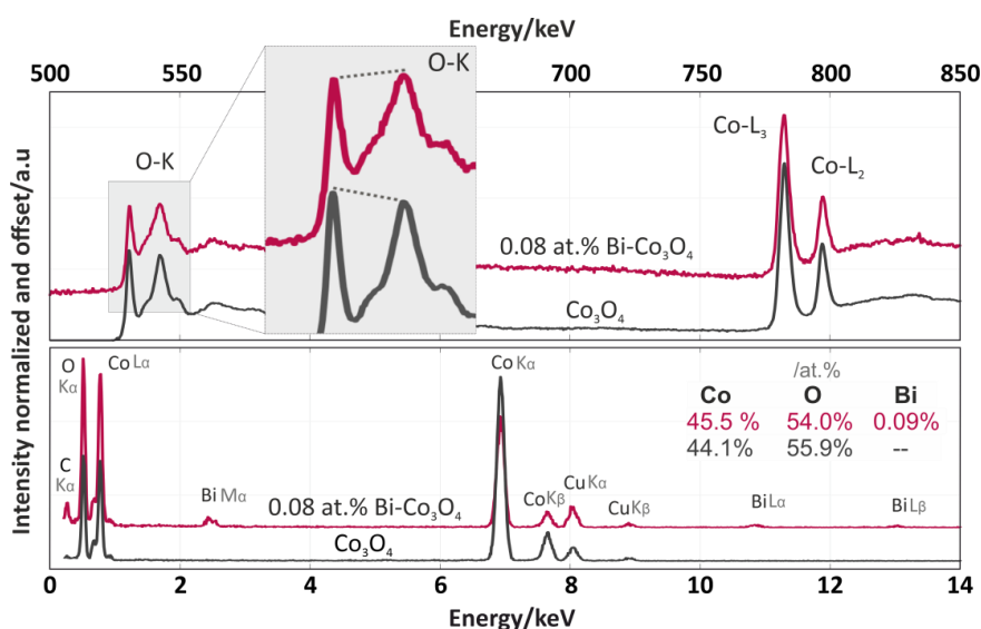
Figure 6. Electron energy-loss spectroscopy (EELS) (upper part) and energy-dispersive X-ray spectroscopy (EDX) (bottom part) spectra of the \text{Co}_3\text{O}_4 (grey) and 6.6 wt % \text{Bi-Co}_3\text{O}_4 (pink) catalysts.
