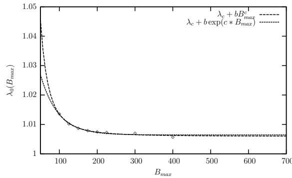
Fig. 3. The fitted dependencies of \lambda_0(B_{\max}) on B_{\max} .
