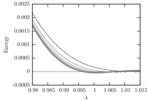
Fig. 2. Polynomials fitted to the dependence of the energy of the ground state in sector with two fermions on the coupling \lambda for different B_{\max} as well as their zero points. The highest dashed curve represents the results for the smallest B_{\max} = 100 , whereas the lowest one corresponds to the highest B_{\max} = 400 .
