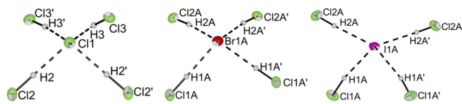
Figure 3. Molecular structure of [PPN][Cl(HCl) 4 ] - , [PPN][Br(HCl) 4 ] - , and [PPN][I(HCl) 4 ] - in the solid state with thermal ellipsoids shown at 50% probability. Cation and disorders have been omitted for clarity (see Figures S5–S9 for representation including cations and disorders). Selected interatomic distances [pm]: Cl2–Cl1 334.8(1), Cl3–Cl1 341.6(1), Cl1A–Br1A 347.7(1), Cl2A–Br1A 354.0(2), Cl1A–I1A 370.4(2), Cl2A–I1A 374.8(2).
