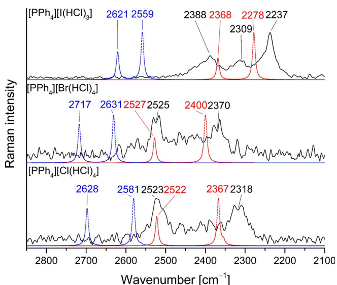
Figure 2. Raman spectra of single crystals of [\text{PPh}_4][\text{X}(\text{HCl})_n] recorded at -196^\circ\text{C} (black) as well as calculated gas phase spectra (B3LYP/def2-TZVPP (red) and MP2/def2-TZVPP (blue)) of [\text{X}(\text{HCl})_n]^- ( n=4 for \text{X}=\text{Cl} , \text{Br} and n=3 for \text{X}=\text{I} ).
