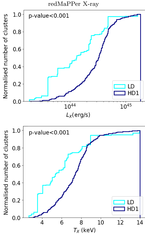
Figure 7. The normalised cumulative X-ray luminosity (top) and temperature (bottom) distributions of redMaPPer X-ray clusters in most underdense (LD) and most overdense (HD1) cluster categories.
