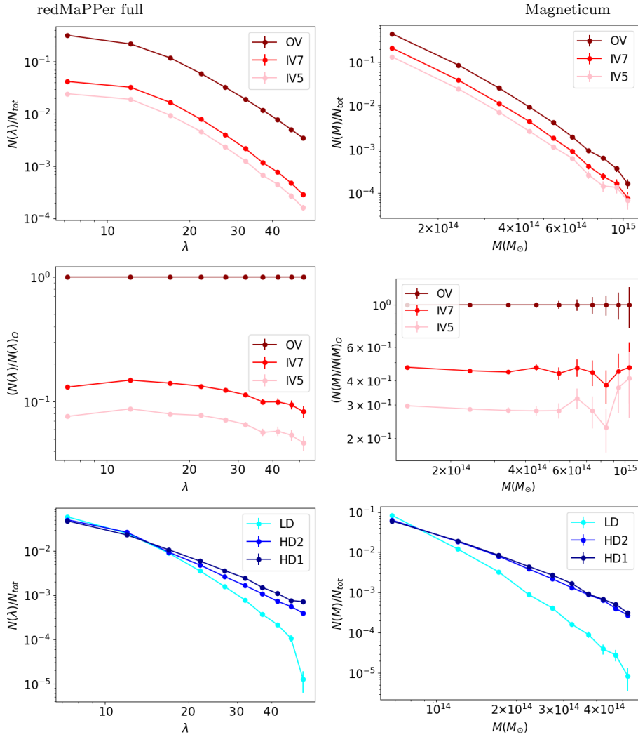
Figure 6. The normalised richness and mass functions of redMaPPer full (left) and Magneticum (right) clusters respectively with respect to the number of all clusters available in OV, IV7 and IV5 categories (top panels), the normalised functions to the number of clusters in OV category (clusters outside voids; middle panels) and the number of all clusters available in LD, HD1 and HD2 categories (bottom panels). It is easier to see the discrepancies of the functions in the high richness/mass end of the top panels in the middle ones. Errors are included in all functions.
