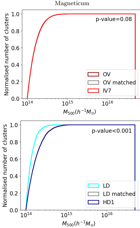
Figure 5. The normalised cumulative mass distributions of Magneticum clusters in IV7 and OV categories (top) and most overdense and most underdense regions (bottom). Once mass distributions are compared, the OV and LD categories are matched to the IV7 and HD1 ones respectively and the p -values of their comparisons are shown on the top of the graphs.
