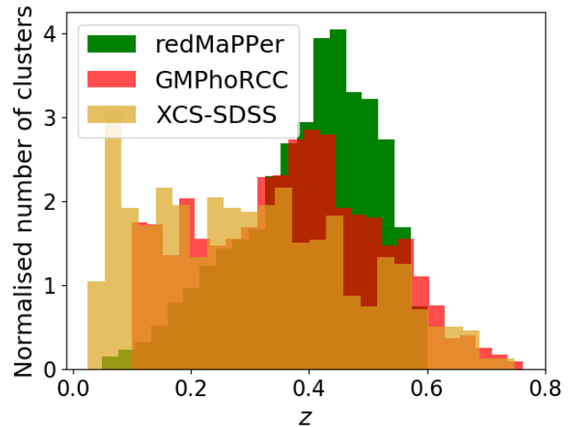
Figure 2. The normalised redshift distributions of the three cluster catalogues. In green, the redMaPPer clusters, in yellow, the XCS DR2–SDSS clusters and in red, the GMPhoRCC clusters.
