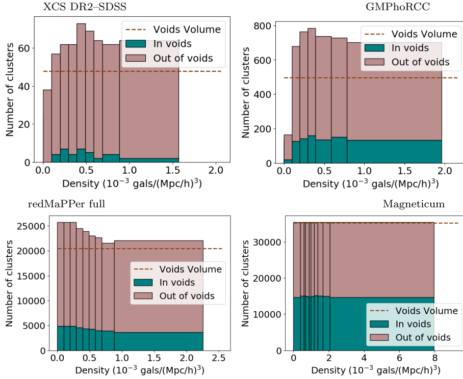
Figure 3. The number of clusters in and out of voids in each density bin for XCS DR2-SDSS (top left), GMPhoRCC (top right), redMaPPer full (bottom left) and Magneticum (bottom right) cluster catalogue. The brown dashed line shows the number of clusters we would expect in voids considering the percentage of the volume survey that are voids.
