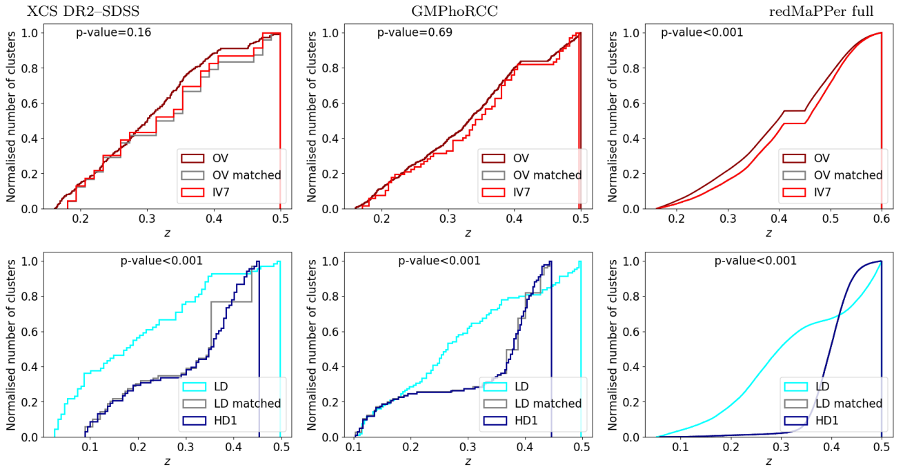
Figure 4. The normalised cumulative redshift distributions of XCS DR2-SDSS (left), GMPhoRCC (middle) and redMaPPer full (right) clusters in IV7 and OV categories (upper panels) and most overdense and most underdense regions (lower panels). Once redshift distributions are compared, the OV and LD categories are matched to the IV7 and HD1 ones respectively and the p-values of their comparisons are shown on the top of the graphs. The redMaPPer matched distributions match the IV7 and HD1 distributions very well and therefore are not distinguishable in the graph.
