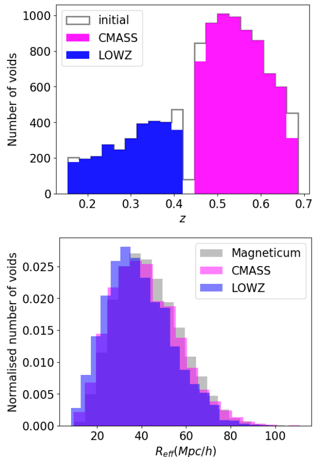
Figure 1. Top panel: In grey, the initial redshift distribution of BOSS void catalogues as taken from Nadathur (2016). The blue and magenta histograms are the redshift-cut distributions of LOWZ and CMASS void catalogues we study respectively. Bottom panel: The effective radius distribution of the voids in the two BOSS catalogues (LOWZ in blue and CMASS in magenta) and in Magneticum voids (grey). The lower galaxy number density in CMASS data results in a void size distribution shifted towards larger effective sizes than for LOWZ.
