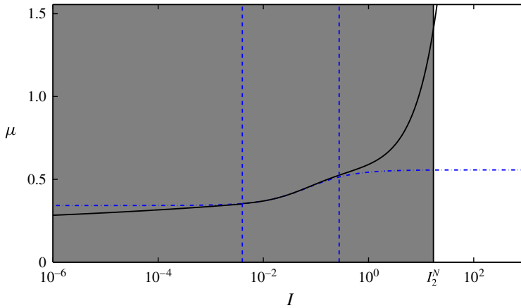
FIGURE 7. The regularised \mu(I) curve (6.3) in black compared with the curve (2.12) of Jop et al. (2005) plotted as the blue dot-dashed curve. The vertical dashed lines are the neutral inertial numbers for \mu_J and the vertical solid line is the maximum well-posed inertial number for the regularised curve.
