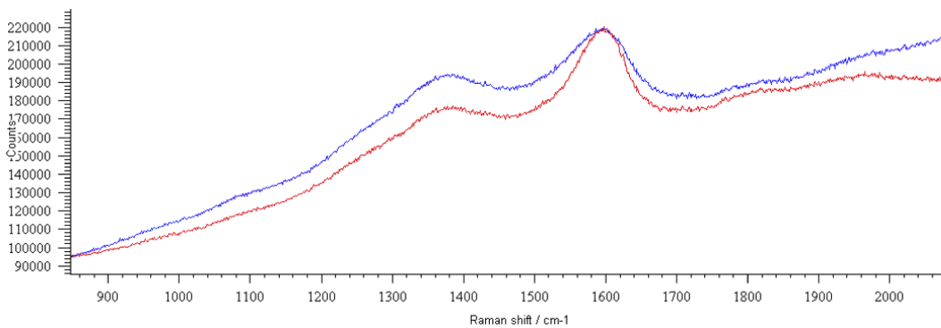
257 Fig. 7 Raman spectrum of a black spot on SF 10541 (red, bottom) and (modern) coal (blue, top).
