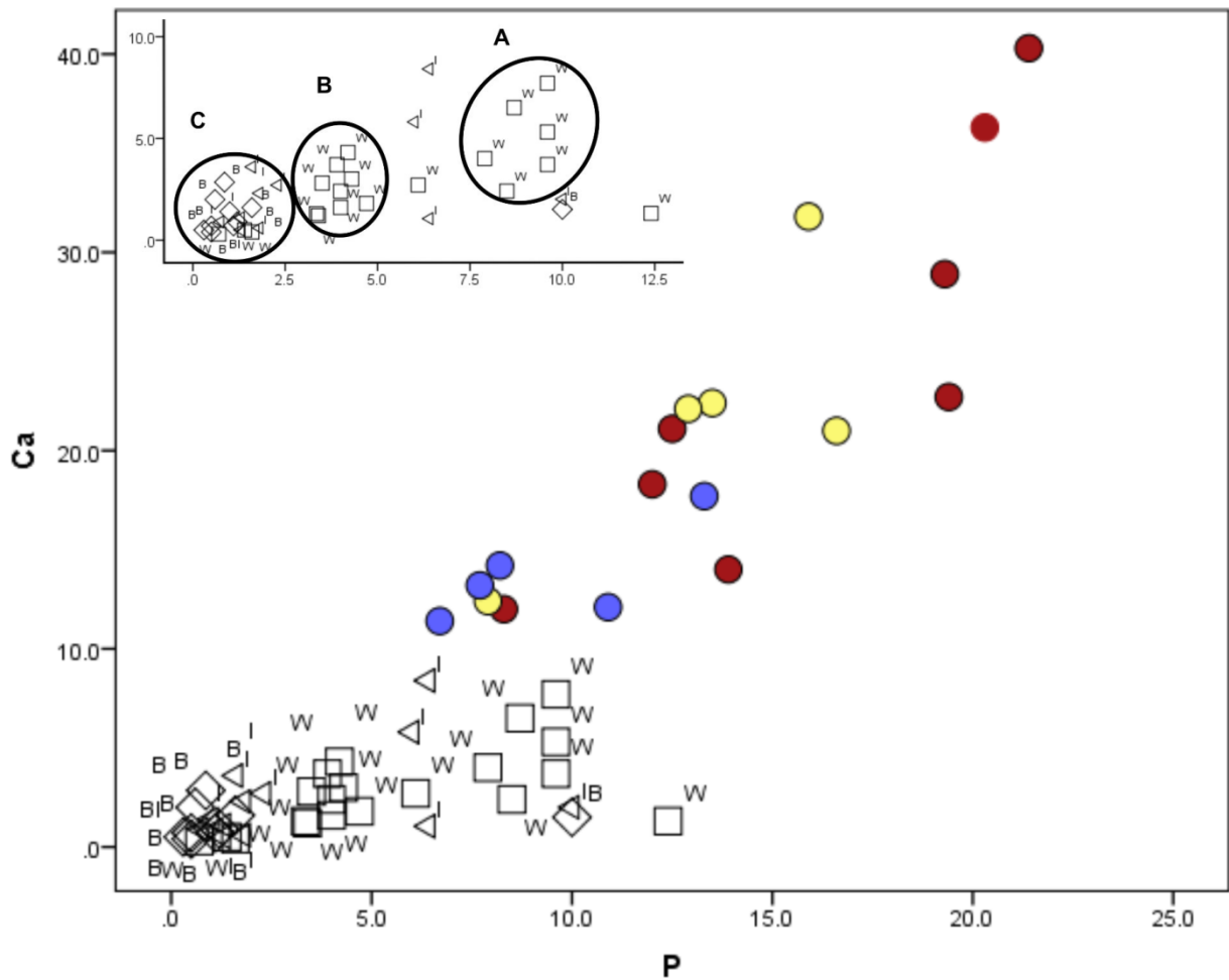
171 Fig. 3 Ca-P plot of examples of white decoration (W), interior surface (I) and body (B) in the 172 decorated sherds; pXRF data. Bone: blue unburnt, yellow carbonised, red calcined. The inset shows 173 Groups A, B and C which represent high, medium and low P respectively.
