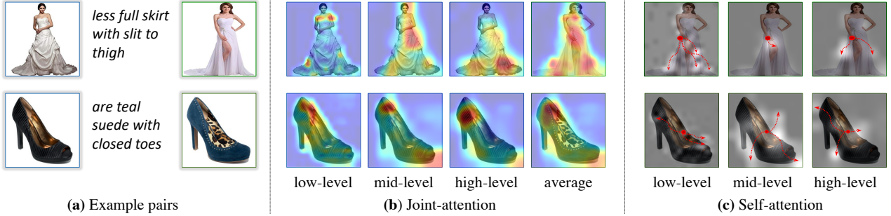
Figure 7. Attention visualisation. (a) Example pairs of reference image, user text as input query, and desired target image output. (b) The attended regions for preservation selected by joint-attention at multi-levels; and the average attended regions across all levels. (c) The self-attention at the central query point, with arrows indicating the attended regions.
