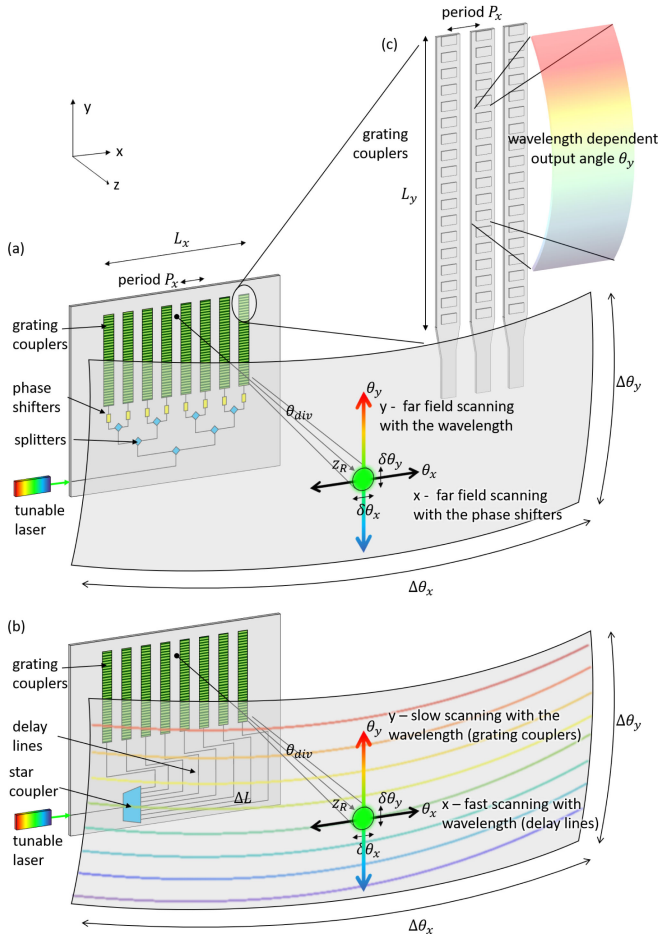
Fig. 1. Basic principle of wavelength steering with an OPA. (a) 1D scanning using active phase shifters and a grating coupler (c) with wavelength dependent output angle [5]. (b) 2D dispersive beam scanning controlled by the wavelength of the input light, as described in [6]. The scanning along the slow y -axis is governed by the dispersion of the antenna (grating coupler), while the scanning along the fast x -axis is governed by the delay length \Delta L .
