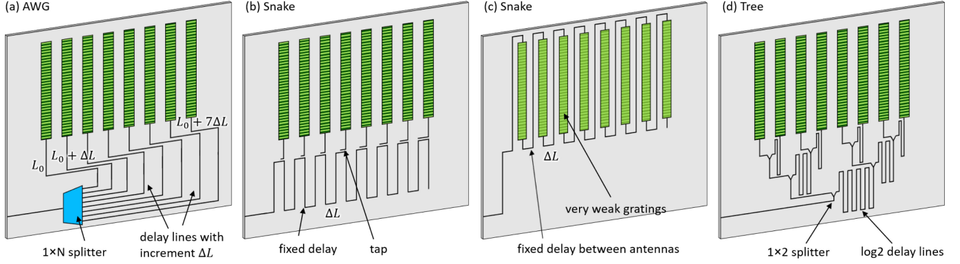
Fig. 2. Different circuit architectures to implement the incremental delays of a DOPA. (a) Arrayed waveguide grating (AWG) where the light is split over N_x waveguides with increasingly long length [6]. (b) Snake, where light is tapped off at fixed distances \Delta L . (c) An alternative implementation of Snake [22], [23], where the grating is part of the delay and taps off the light directly. (d) Imbalanced splitter tree, where in each stage m a delay 2^m \cdot \Delta L is added in one arm.
