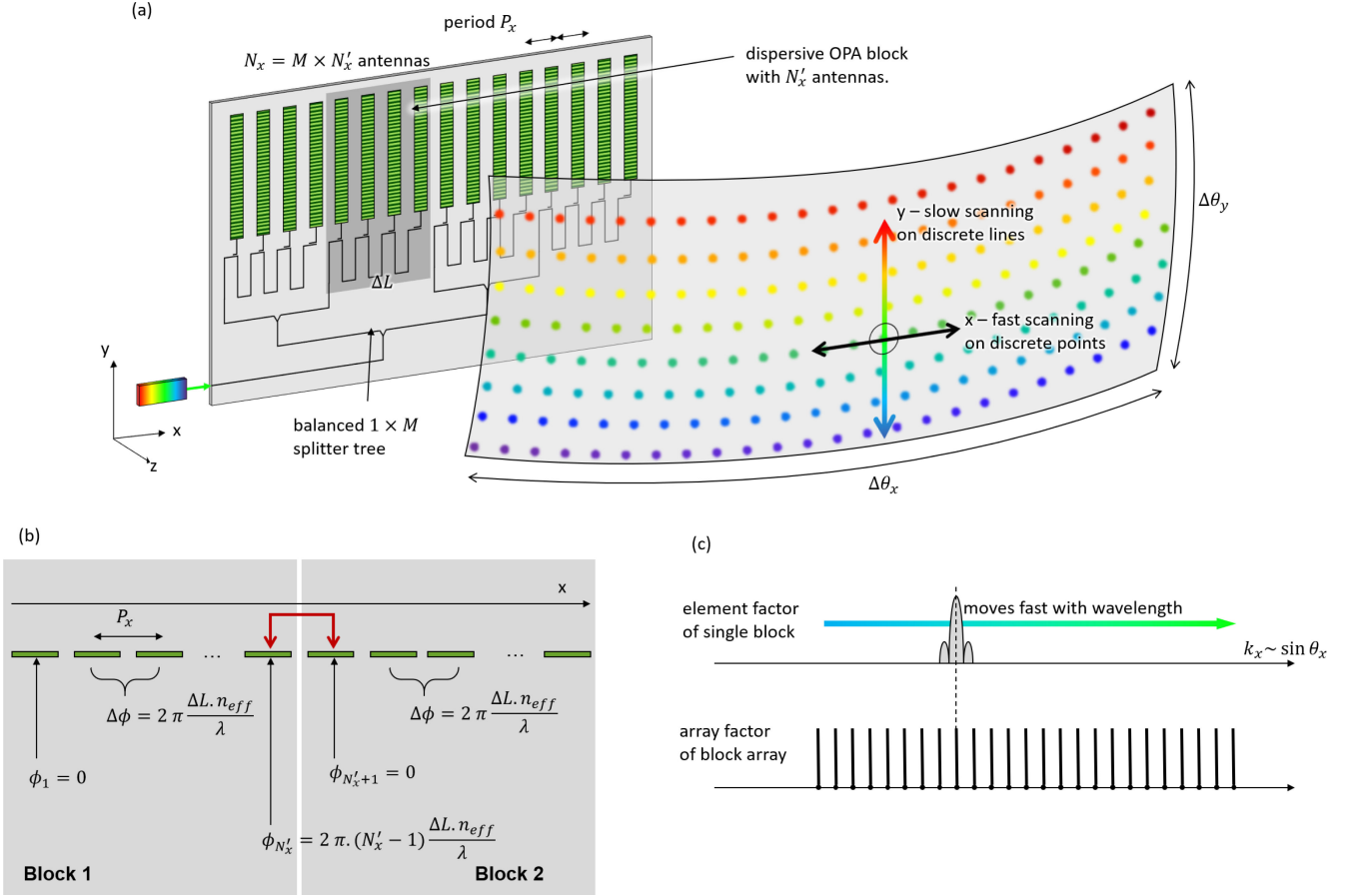
Fig. 5. Discretized dispersive optical phased array. (a) Schematic structure, where each block consists of a snake-like OPA. It is also possible to use a Tree or AWG-like OPA in each block. (b) Condition when all antennas are in phase, and (c) overlap of scanning beam of single block with diffraction orders of the large array.
