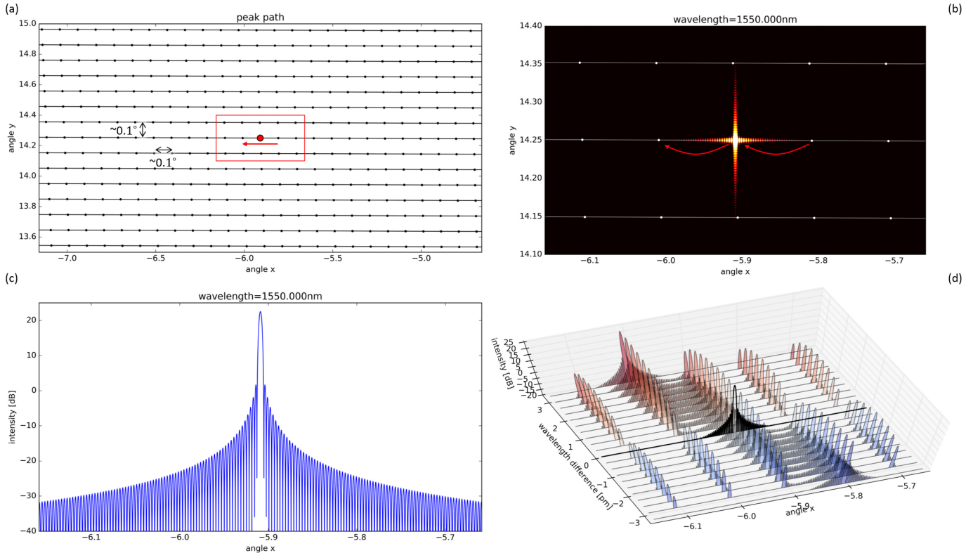
Fig. 6. Simulated farfield of the pixelated dispersive OPA, with similar antenna amplitudes (Gaussian distribution) as the dispersive OPA from Fig. 4. (a) Trajectory of the peak in the far field, with the conditions for constructive interference. (b) Farfield intensity (in dB) at the peak indicated with the red dot in (a). (c) Cross section along \theta_y of the field in (b). (d) Evolution of the \theta_x far field as function of wavelength along the red arrow in (a)–(b). We have included a supplementary MP4 video illustrating the farfield scan as function of wavelength. This is available at https://ieeexplore.ieee.org/document/9170765/media#media .
