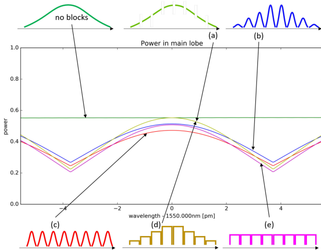
Fig. 8. Power in the main lobe for the different implementations of the dispersive OPA, depicted in Fig. 4, 6 and 7.
