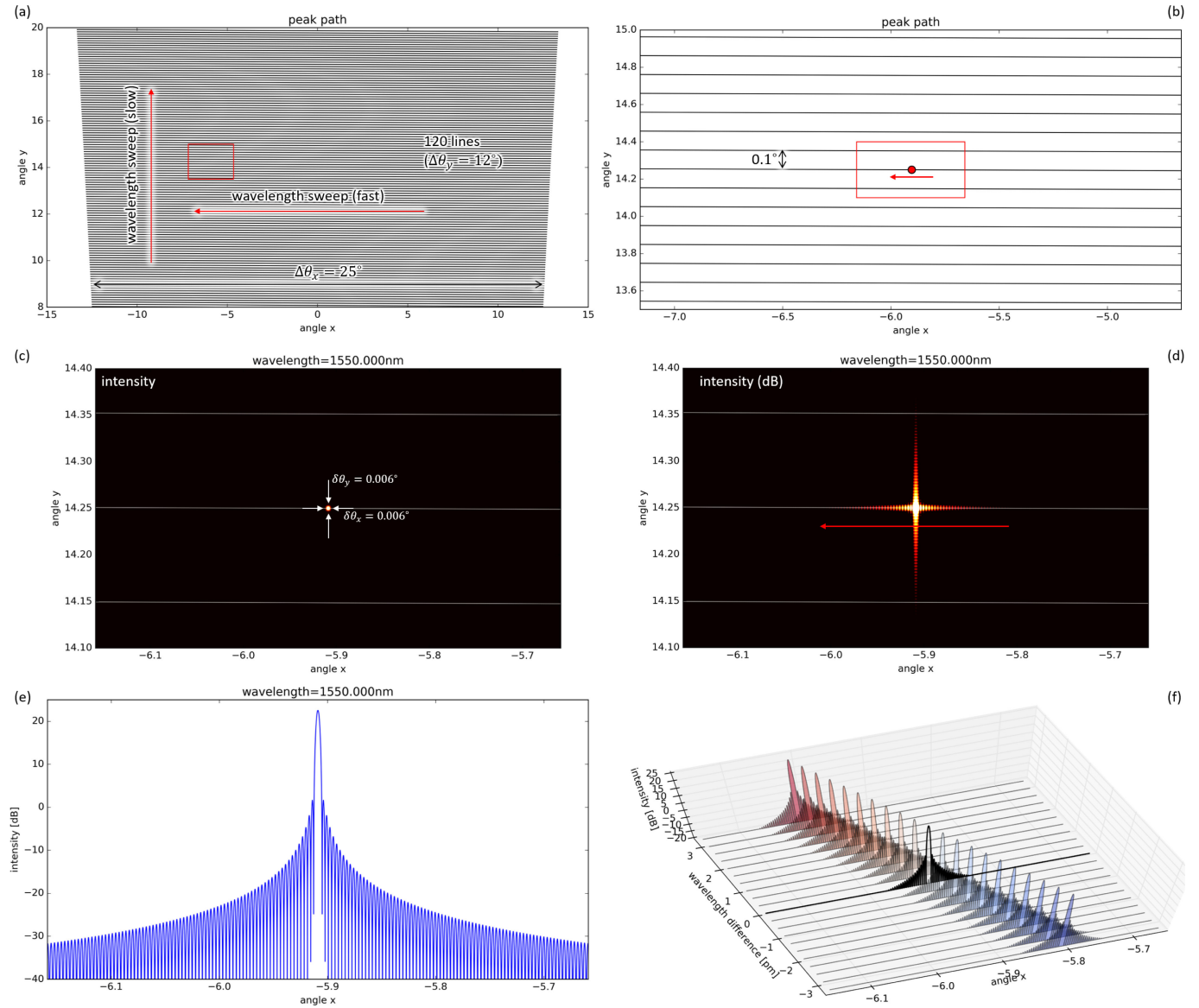
Fig. 4. Simulation of a dispersive OPA with design parameters from Table I. (a) path of the projected beam in the far field for a wavelength scan. (b) Detail of the path within the red box of (a). (c) Close-up of the farfield image at a single wavelength within the red box indicated in (b), (d) Same far-field, plotted in dB, (e) Cross section of the far field along \theta_x , plotted in dB, (f) Progress of the \theta_x far field profile as function of wavelength for a 6.4 pm wavelength range. We have included a supplementary video illustrating the farfield scan as function of wavelength. This is available at https://ieeexplore.ieee.org/document/9170765/media#media .
