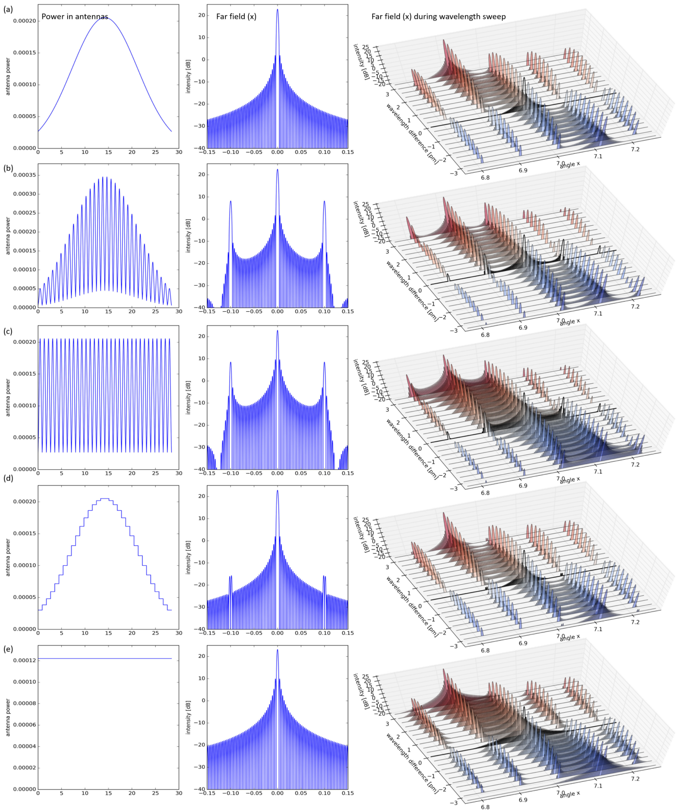
Fig. 7. Different power distribution profiles for the pixelated dispersive OPA, the resulting far field profile when all the antennas are in phase, and the evolution of the far-field when sweeping the wavelength. (a) Gaussian profile over all antennas, as used in Fig. 6. (b)–(e) Different combinations of Gaussian and Uniform distributions within a block and between blocks. All power distributions are normalized for unity power.
