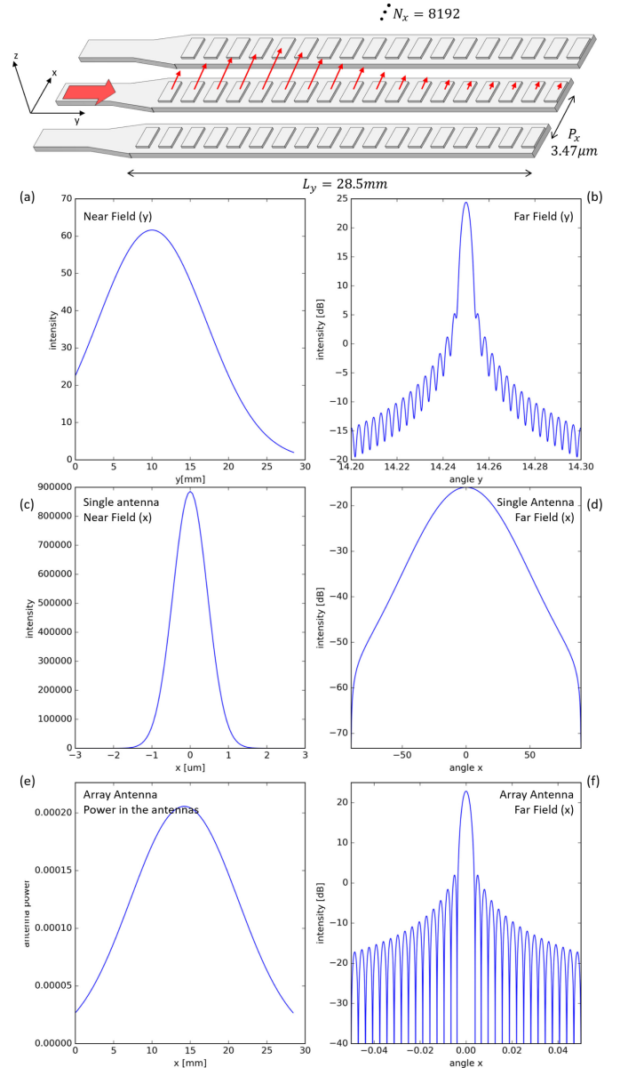
Fig. 3. Field profile of the antenna used for the simulation example. (a)–(b) Near-field/far-field above a single antenna along the y/\theta_y direction. (c)–(d) Near-field/far-field above a single antenna along the x/\theta_x direction. (e) Amplitudes of the individual antennas along the x direction. (f) Far-field of the array antenna along \theta_x when all the elements are in phase.
