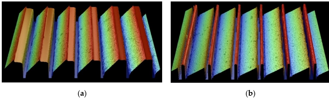
Figure 6. Hot embossed structures on PMMA coated ITO glass with (a) a press force of 20 kN at 145 ^{\circ}\text{C} for 120 s; (b) a press force of 25 kN at 165 ^{\circ}\text{C} for 200 s.
