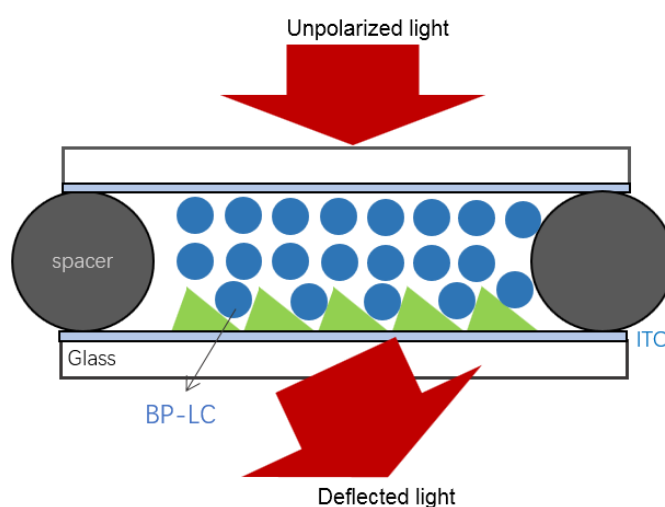
Figure 24. Schematic BP LC-micro grating based beam steering device.
