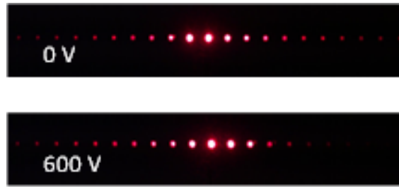
Figure 25. Laser beam ( \lambda = 633 \text{ nm} ) steering patterns without and with applied voltages. Reproduced with permission [91]. Copyright 2017, Photonics Society of Poland.
