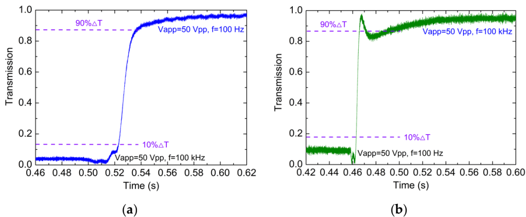
Figure 23. The switching time of the DF NLC beam steering device by applying V_{app} = 50 V_{pp} : (a) with f = 100\text{ kHz} \rightarrow 100\text{ Hz} ; (b) with f = 100\text{ Hz} \rightarrow 100\text{ kHz} . Reproduced with permission [88]. Copyright 2019, IOP Publishing.
