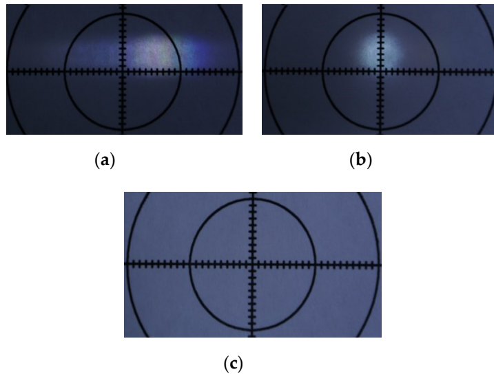
Figure 19. White light beam deflection by Ch-LC beam steering device: (a) P state; (b) H state; (c) FC state. Reproduced with permission [87]. Copyright 2017, Nature Publishing.
