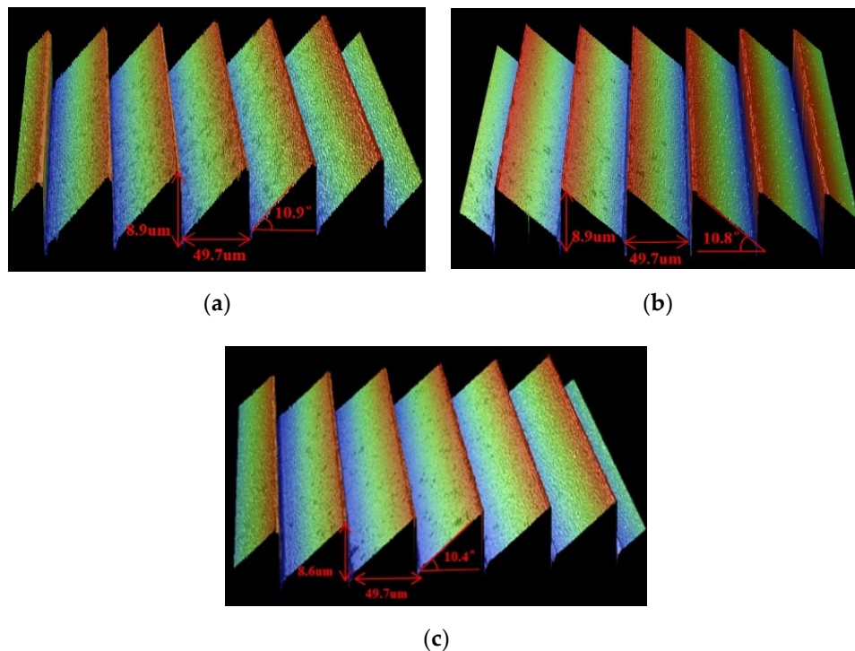
Figure 11. Surface profile characterized by a WYKO surface profiler: (a) master grating on PMMA sheet; (b) negative PDMS mold; (c) NOA 74 grating replica. Reproduced with permission [63]. Copyright 2015, IEEE.
