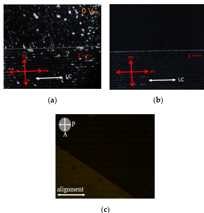
Figure 13. LC textures within the LC-micro grating devices by different alignment technologies: (a) velvet rubbing; (b) oblique SiO 2 evaporation; (c) photo-alignment. Reproduced with permission [63], copyright 2015, IEEE; reproduced with permission [64], copyright 2016, OSA.
