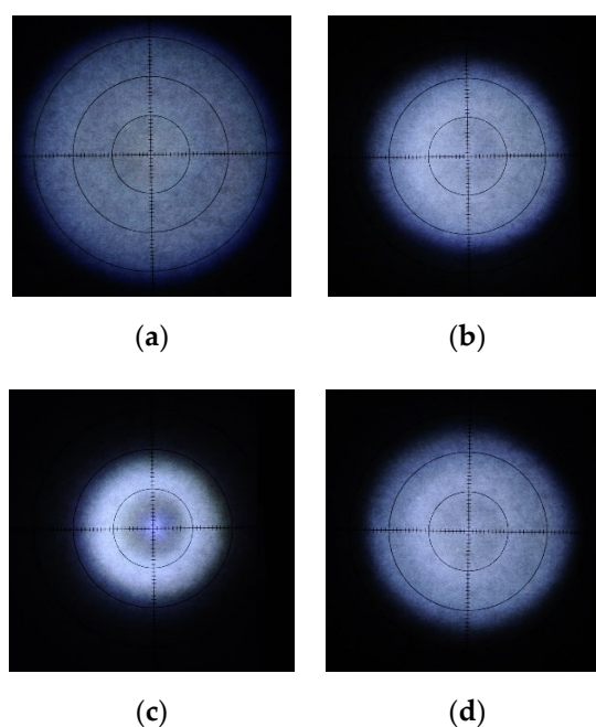
Figure 16. Circular beam shaping of LC-CMG devices with a white LED and a polarizer: (a) V = 0 V_{pp} and (b) V = 50 V_{pp} for the LC beam broadening device; (c) V = 0 V_{pp} and (d) V = 50 V_{pp} for the LC beam condensing device. Reproduced with permission [77]. Copyright 2016, IOP Publishing.
