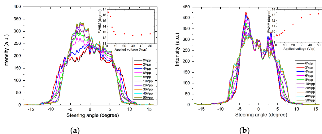
Figure 17. Plots of the intensity distribution as a function of angle for (a) LC beam broadening device and (b) LC beam condensing device. Reproduced with permission [77]. Copyright 2016, IOP Publishing.
