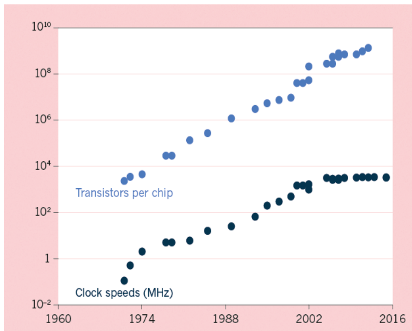
Figure 1: A plot showing the relationship between clock speed and transistors per chip over the last 50 years. (Waldrop, 2016)
