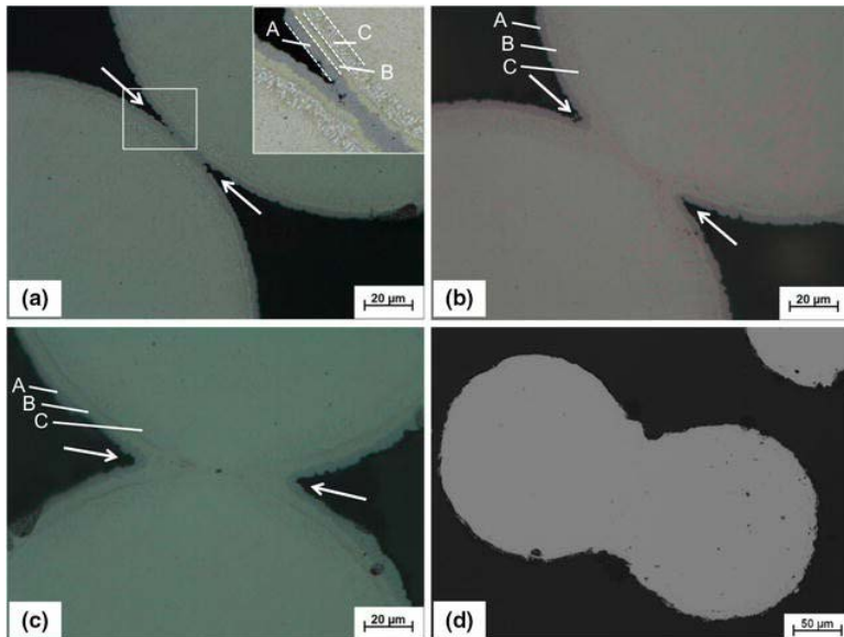
Fig. 1 Optical micrographs of the cross sections of bonded wire pairs after aluminotitanizing by pack cementation for (a) 15 min, (b) 30 min, and (c) 60 min, showing increasing bonding area and cusp radii (arrows) and increasing coating thickness (A: \text{Ni}_2\text{AlTi} , B: \text{Ni}_3(\text{Al,Ti}) , and C: Rejected Cr in \gamma ). (d) Pair of wires after a full heat treatment (aluminotitanized for 60 min, TLP-bonding and homogenization, solutionizing and aging), showing increased bonding area and disappearance of the coating layers seen in (a) through (c)
