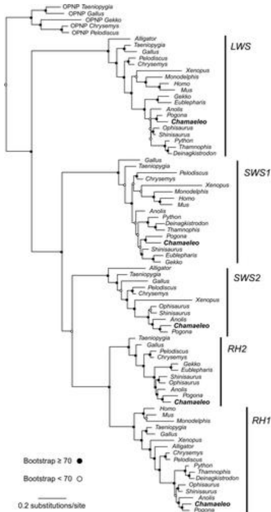
Figure 1 A maximum-likelihood phylogenetic reconstruction of the visual opsins of C. calyptratus and other tetrapods, including: vertebrate rhodopsin (RH1), long wavelength-sensitive opsin (LWS), short-wave sensitive 1 (SWS1), short-wave sensitive 2 (SWS2), and RH1-like 2 (RH2)
