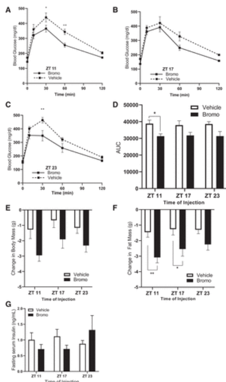
Fig. 6. Bromocriptine (Bromo) injections in diet-induced obese (DIO) Zeitgeber time (ZT) mice at ZT 11 and ZT 23 improves glucose tolerance. A: Bromo treatment (solid line) at ZT 11 improves glucose clearance compared with vehicle (dashed line) in response to a glucose tolerance test (2 mg/kg). B: Bromo treatment (solid line) at ZT 17 does not improve glucose clearance compared with vehicle (dashed line) in response to a glucose tolerance test (2 mg/kg). C: Bromo treatment (solid line) at ZT 23 improves glucose clearance compared with vehicle (dashed line) in response to a glucose tolerance test (2 mg/kg). A–C: * P < 0.05 , ** P < 0.01 . Repeated-measures ANOVA
