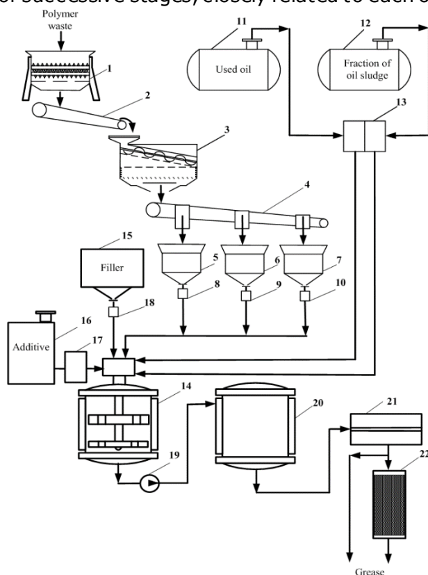
Fig. 1. The scheme for obtaining recycled grease: 1 – chopper; 2, 4 – belt conveyors; 3 – apparatus for washing and drying polymer waste; 5-7, 15 – bunkers; 8-10, 18 – dispensers; 11, 12, 16 – tanks; 13, 17 – dosing pumping devices; 14 – reactor; 19 – pump; 20 – cold-storage space; 21 – homogenizer; 22 – filter
