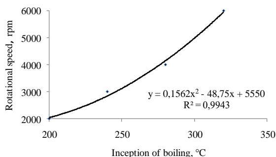
Fig. 3. The dependence between the rotational speed of the centrifuge and the inception of boiling of the degradation fraction of polyethylene raw materials
