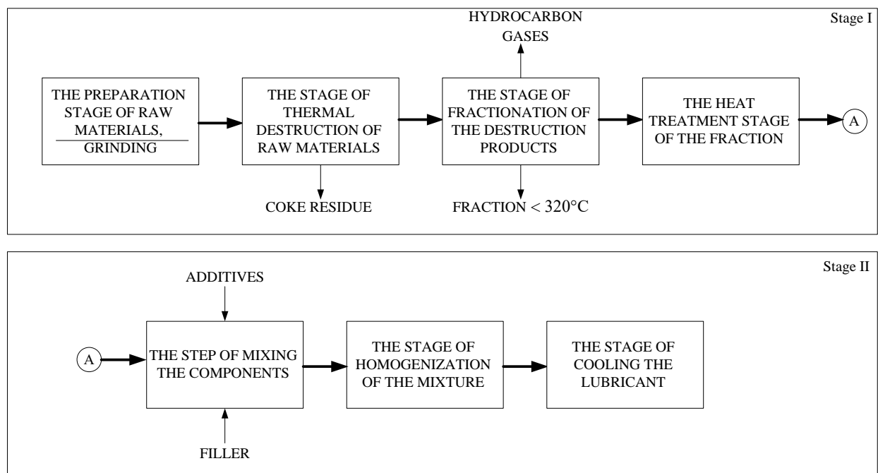
Fig. 4. The scheme for the grease production from secondary polyethylene raw materials
