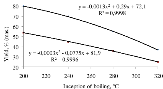
Fig. 2. The dependence between the yield and the inception of boiling of the degradation fractions of polyethylene raw materials: 1-output for raw materials; 2- broad band outlet
