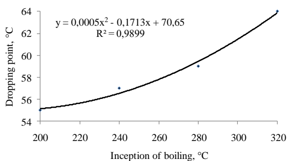
Fig. 1. The dependence between the dropping point and the inception of boiling fractions of polyethylene raw material destruction
