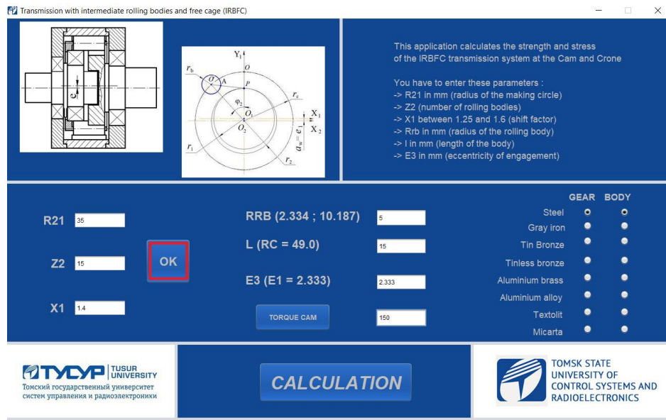
Figure 4. Introduction of initial and additional parameters for calculating forces and contact stresses.
