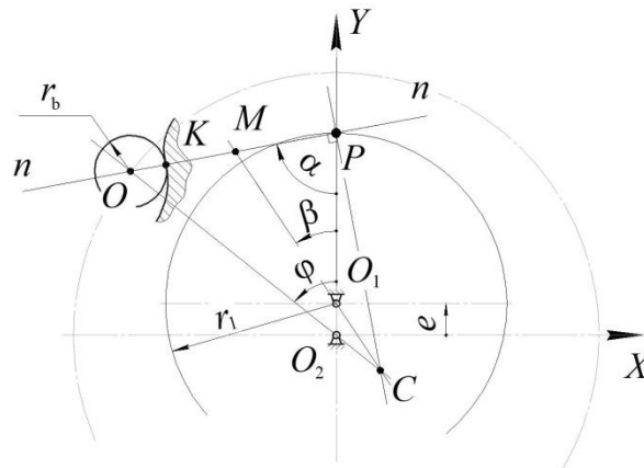
Figure 2. For cam profile to the determination of the radius of curvature.
