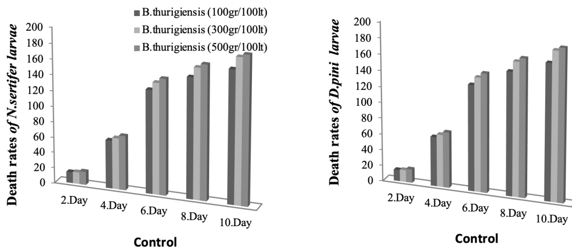
Fig. 2. The effectiveness of different doses of Dipel® DF BT on the larvae of N. sertifer and D. pini .
