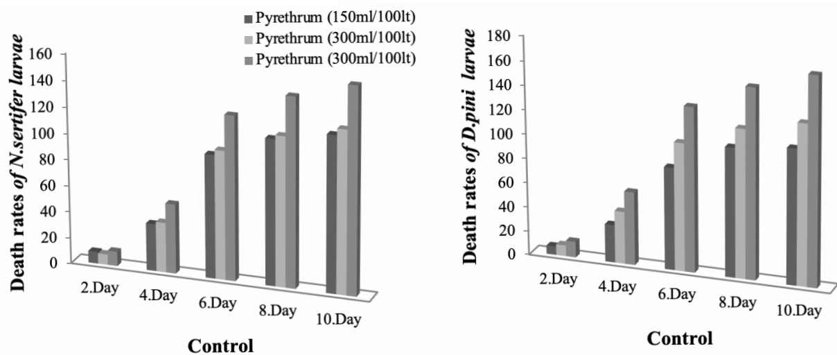
Fig. 1. The effectiveness of different doses of Pyrethrum on the larvae of N. sertifer and D. pini .
